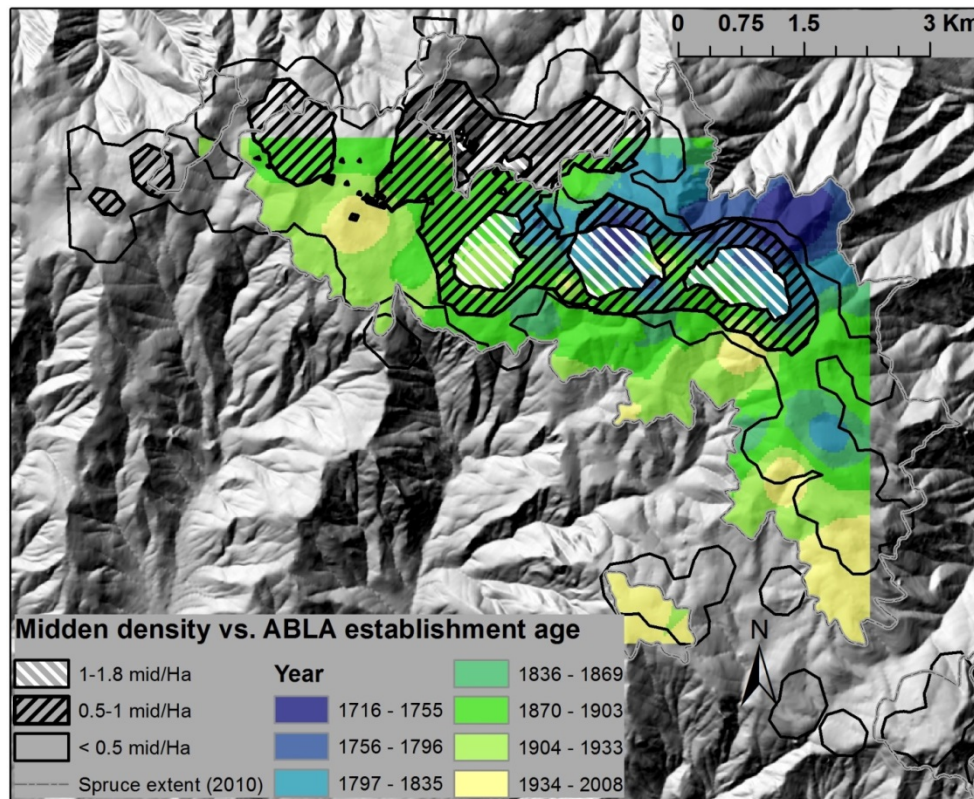
Figure S-2 Midden density overlaid on Corkbark fir establishment. The colored extent is limited to the forested area above 2,835 m elevation. The corkbark fir age surface is interpolated from 37 gridded point locations. Spatial interpolation is based on an inverse distance weighting algorithm that uses four nearest point locations with a power function of two (O'Connor et al. 2013). The midden density surface is generated from 1033 midden locations in the year 1996.
