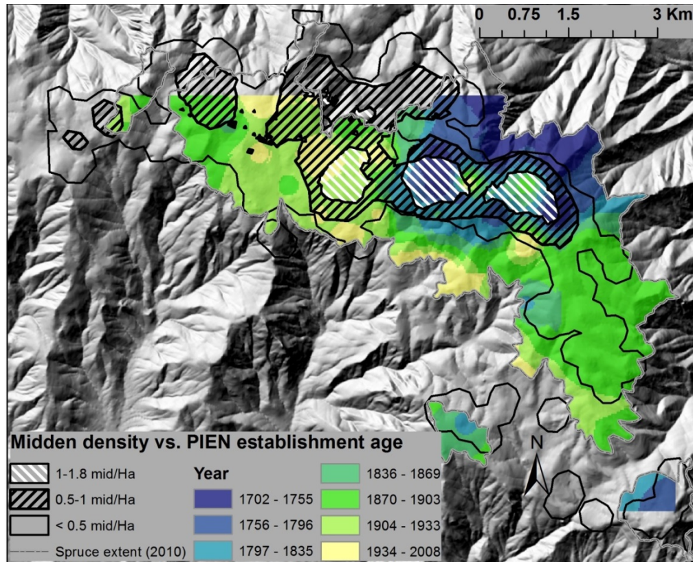
Figure S-1 Midden density overlaid on Engelmann spruce establishment. The colored extent is limited to the forested area above 2,835 m elevation. The spruce age surface is interpolated from 44 gridded point locations. Spatial interpolation is based on an inverse distance weighting algorithm that uses four nearest point locations with a power function of two (O'Connor et al. 2013). The midden density surface is generated from 1033 midden locations in the year 1996.
