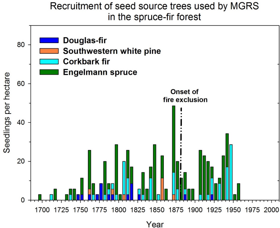
Figure 2 Seedling recruitment in spruce-fir forest from 1685 through 2008. Seedling recruitment demonstrates periodic pulses related to disturbance from spruce beetle outbreaks (N = 6, 0.05-ha plots). In contrast to the mixed-conifer forest, recruitment does not appear to be affected by EuroAmerican settlement in the 1880s. A trend of increasing domination of recruitment by corkbark fir and Engelmann spruce can be seen by the mid-1800s. Low seedling recruitment after 1950 suggests that the spruce-fir forest was fully stocked prior to the series of insect outbreaks and fires of the 1990s.
