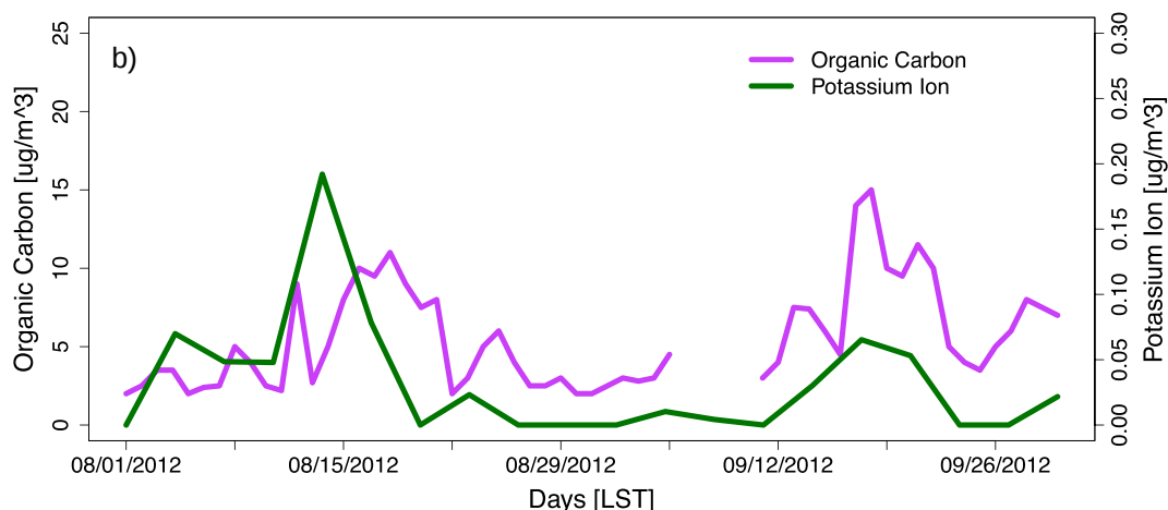
Figure 12. (a) Modeled and observed daily averaged PM 2.5 concentrations at SLC. (b) Measured values of organic carbon (daily) and speciated potassium ion concentrations (every 3 days) at SLC.
