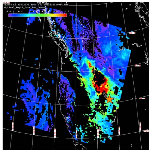
Figure 14. Aerosol optical depth as retrieved from MODIS-TERRA, observed at the same time as shown in Figure 13. The star indicates the location of SLC. Credit: NASA.
