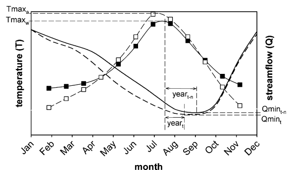
Fig. 1 Conceptual model of the hypothesized shift in timing of biologically relevant hydro-climatic variables affecting streams in Western North America between the years t and t - n . The figure represents the seasonal distribution for monthly mean values of stream flow for the year t - n (solid line), the hypothesized stream flow for the year t (dotted line), the stream temperature (solid line with filled symbols), and the air temperature (dotted line with open symbols). The lag between the annual stream temperature maxima ( T_{\max,w} ) and the annual stream flow minima ( Q_{\min} ) is shown for the year's t and t - n
