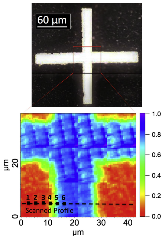
Fig. 8. (top) Optical image of photo lithographically patterned gold black with 150 nm of SiO 2 thick protection layer (dark) on gold substrate (bright). (bottom) Integrated infrared reflectance of gold black pattern (900 to 3700 cm -1 ). The infrared image is a mosaic formed by stitching 4 × 3 hyper-spectral tiles.
