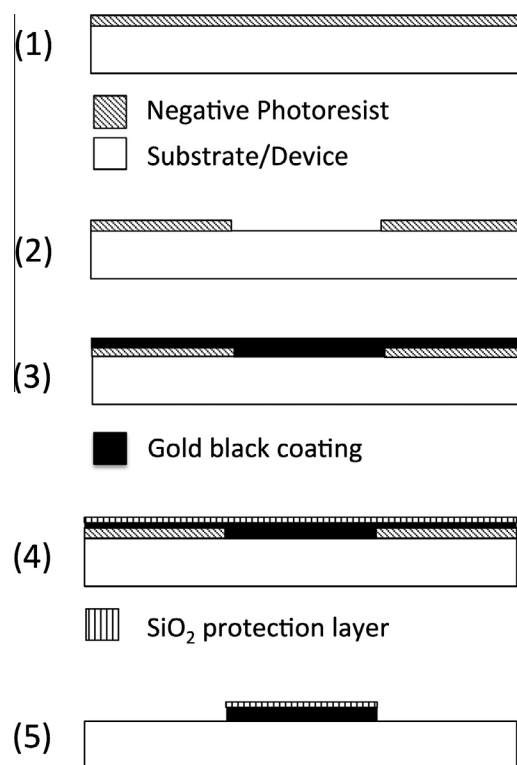
Fig. 1. Schematic of processing sequence patterned gold black/SiO 2 composites.
