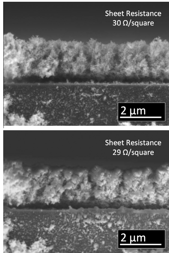
Fig. 4. Cross-sectional SEM images of gold black before (top) and after (bottom) \text{SiO}_2 deposition.
