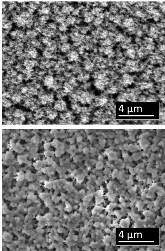
Fig. 3. SEM top-view images of gold black coating before (top) and after (bottom) \text{SiO}_2 deposition.
