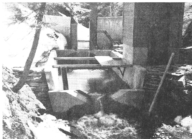
Figure 10.—Spring runoff from one of the Sturgis Watersheds. Station is a tandem San Dimas flume for measurement of high flows and a 120° V-notch weir for measurement of low flows.
