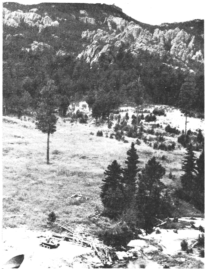
Figure 2.—Typical terrain in the granite "core" of the Black Hills. High point in center background is Harney Peak, the highest in the Black Hills (7,242 feet). Soil lacks cohesion and is highly erosive.
