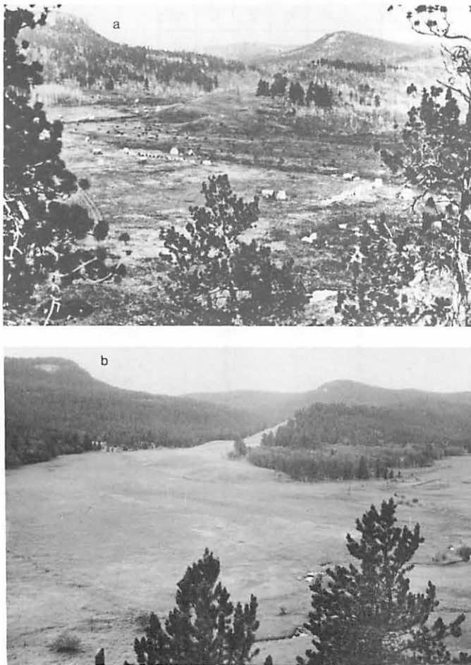
Figure 32.—The view is upstream from Castle Creek. Photograph (a) was taken from one of the Custer camps in 1874. Note the sparse vegetation on the slopes in the background. Photograph (b) was taken from the same location in 1974. Control of fire has been primarily responsible for the development of the forests. Populus tremuloides on the right has matured and probably is climax at that location. The riparian Salix spp. vegetation evident in the foreground in 1874 is completely gone in 1974.
