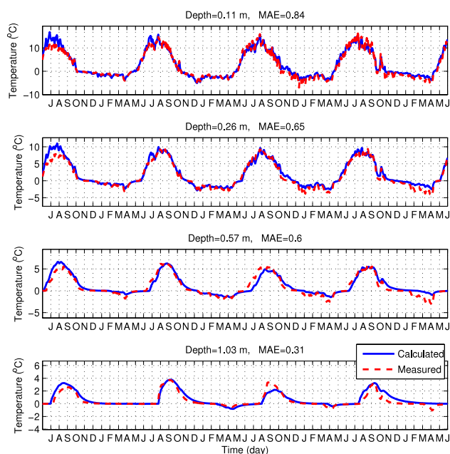
Figure 3. Simulations of the measured ground temperatures at a burned site from June 2000 to June 2004.
