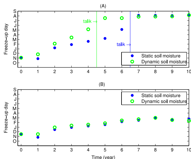
Figure 10. Freeze-up time at (A) the upland black spruce forest site after 15 cm of the organic layer was removed and (B) the lowland black spruce forest site after 48 cm of the organic layer was removed. Here 0 is a year corresponding to the upper organic layer removal.
