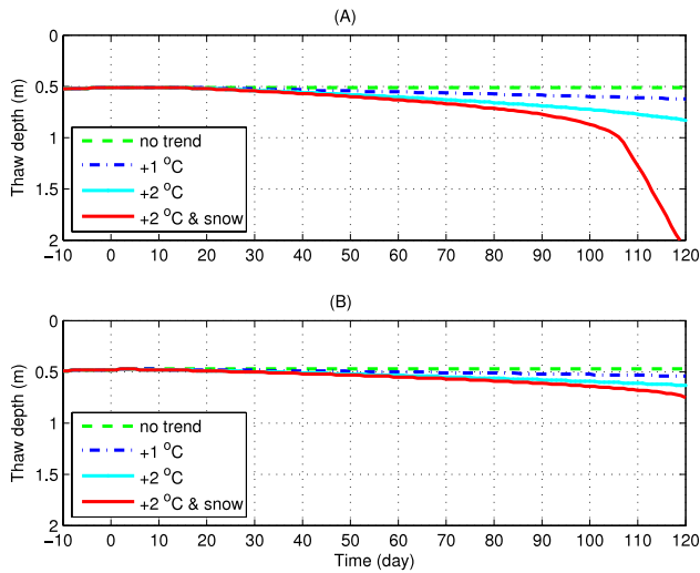
Figure 5. Simulations of the active layer thickness for (A) upland and (B) lowland black spruce forest sites for different warming scenarios with no fire disturbances. Time interval [-10, 0] corresponds to the equilibrium run, and [0, 120] corresponds to the transient run.
