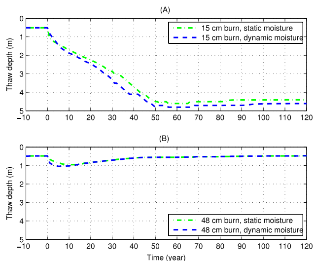
Figure 8. Simulated permafrost table dynamics with and without changes in the soil moisture content within 10 years after fire for (A) upland and (B) lowland sites under the baseline climate scenario (mean annual air temperatures -2^{\circ}\text{C} ) using dynamic organic soils recovery rates generated by the Dynamic Organic Soil Terrestrial Ecosystem Model. Time interval [-10, 0] corresponds to the equilibrium run, and [0, 120] corresponds to the transient run, where 0 is a year corresponding to the upper organic layer removal.
