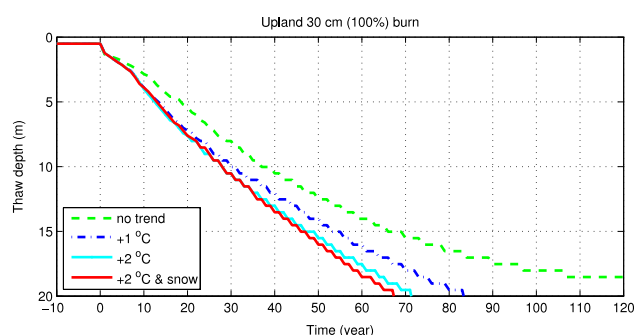
Figure 12. Simulated permafrost table dynamics after 100% of the organic layer was removed in fire at the upland black spruce forest site for different climate warming scenarios using dynamic organic soils and changes in soil moisture content. Time interval [-10, 0] corresponds to the equilibrium run, and [0, 120] corresponds to the transient run, where 0 is a year corresponding to the upper organic layer removal.
