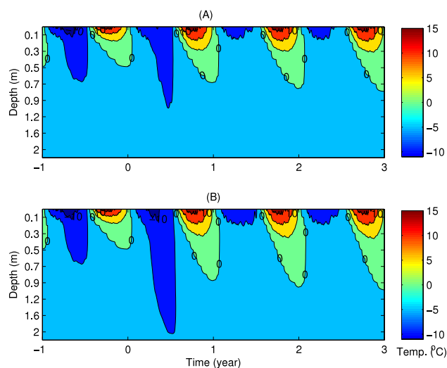
Figure 9. Contour plots of the ground temperature dynamics with depth over time for the lowland black spruce forest site simulated (A) with and (B) without changes in the soil moisture content. Here 0 is a year corresponding to the upper organic layer removal.
