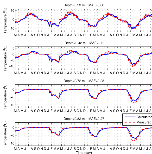
Figure 4. Simulations of the measured ground temperatures at an unburned site from March 1996 to August 1999.
