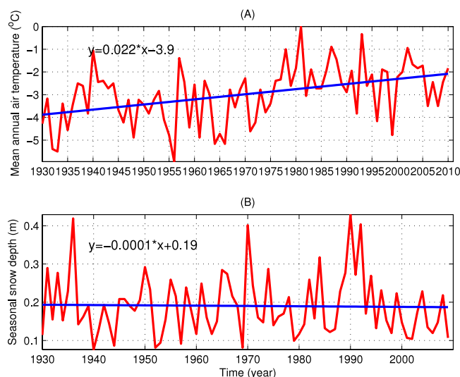
Figure 1. Climatological data from the Fairbanks International Airport station: (A) mean annual air temperature in °C and (B) seasonal averaged snow depth in meters. ACRC: Alaska Climate Research Center, Fairbanks Alaska Climatology, Geophysical Institute, Univ. of Alaska Fairbanks, AK, http://climate.gi.alaska.edu , 2010.
