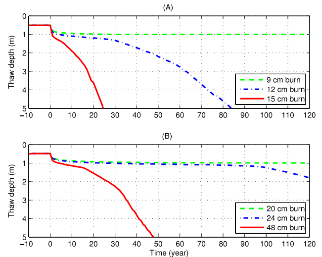
Figure 6. Simulations of the permafrost table depth for (A) upland and (B) lowland boreal spruce forest sites for different fire severities under baseline climate scenario (mean annual air temperatures -2^{\circ}\text{C} ), for no organic layer regrowth. Time interval [-10, 0] corresponds to the equilibrium run, and [0, 120] corresponds to the transient run, where 0 is a year corresponding to the upper organic layer removal.
