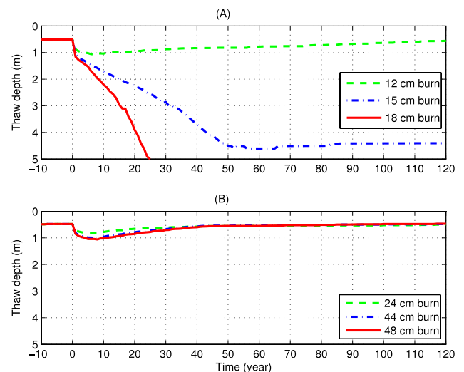
Figure 7. Simulations of the permafrost table depth for (A) upland and (B) lowland boreal forest sites for different fire severities under the baseline climate scenario (mean annual air temperatures -2^{\circ}\text{C} ) using dynamic organic soils recovery rates. Time interval [-10, 0] corresponds to the equilibrium run, and [0, 120] corresponds to the transient run, where 0 is a year corresponding to the upper organic layer removal.
