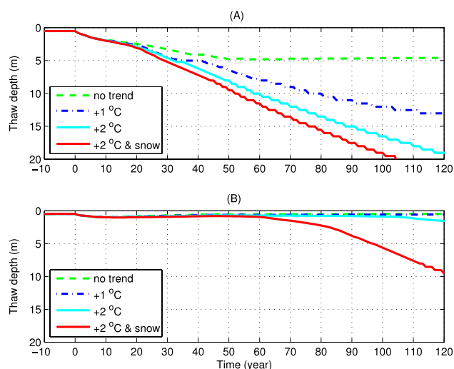
Figure 11. Simulated permafrost table dynamics after (A) 15 cm of the organic layer removed in fire at the upland black spruce forest site and (B) 48 cm of the organic layer removed in fire at the lowland black spruce forest sites for different climate warming scenarios using dynamic organic soils recovery rates and changes in soil moisture content. Time interval [-10, 0] corresponds to the equilibrium run, and [0, 120] time interval corresponds to the transient run, where 0 is a year corresponding to the upper organic layer removal.
