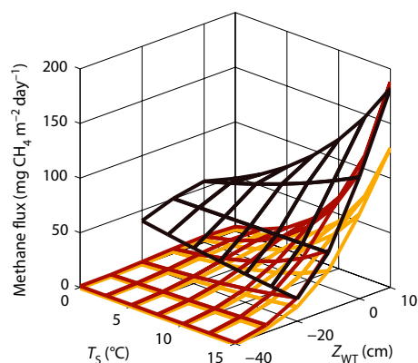
Fig. 7 Visualization of the best model from the regression analysis, after re-transforming to CH 4 flux (mg CH 4 m -2 d -1 ) from log(F CH4+5 ). Upper dark red grid represents the model when applied to sites with a dominant sedge cover; middle bright red grid represents sites where sedges are present and lower yellow grid represents sites where sedges are absent. The visualization is truncated for Z WT < -20 cm for sites with a dominant sedge cover due to few representative sites.
