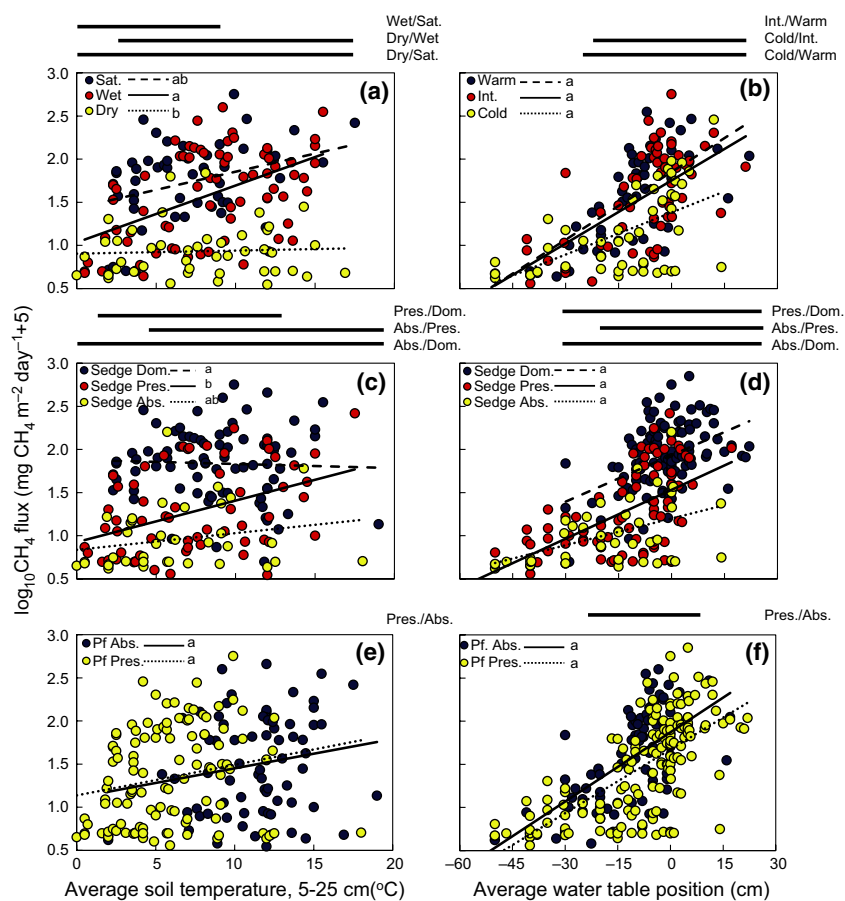
Fig. 6 Visualization of covariance analyses (ANCOVA). Analyses were based on site CH 4 flux being the response variable (represented by \log(F_{CH_4+5}) , where F_{CH_4} is in \text{mg CH}_4 \text{ m}^{-2} \text{ d}^{-1} ), while average water table positions or soil temperatures measured between 5 and 25 cm below the surface were covariates (shown on x-axes). Factors were either soil temperature categories (Cold, Intermediate, or Warm sites, with category separations at 5 and 10 °C), water table categories (Dry, Wet, or Saturated sites with category separations at -15 and -2.5 cm), sedge cover (Dominant, Present or Absent) or permafrost conditions in the upper 2 m (Present or Absent). Bars above each graph indicate the range over which pairs of factors are significantly different, based on 95% confidence intervals of fits. Lower case letters following the legend indicate differences ( P < 0.05 ) for the slopes of the fits, based on Tukey HSD test. See Supplemental information for detailed ANCOVA statistics.
