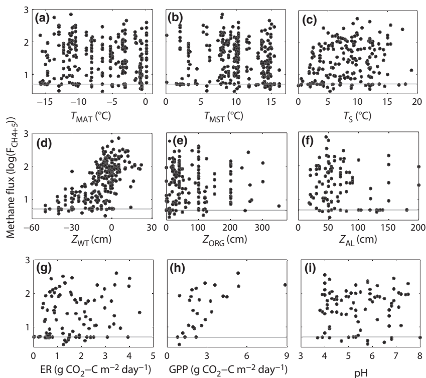
Fig. 2 Relationships between site average growing season \text{CH}_4 flux (expressed as \log(F_{CH_4+5}) , where F_{CH_4} is in \text{mg CH}_4 \text{ m}^{-2} \text{ d}^{-1} ), environmental variables and \text{CO}_2 fluxes; long-term mean annual air temperature ( T_{MAT} ), long-term mean summer temperature ( T_{MST} ), mean soil temperature measured between 5 and 25 cm below the surface ( T_S ), mean water table position ( Z_{WT} ), depth of the organic soil layer ( Z_{ORG} ), depth of the active layer ( Z_{AL} ), mean ecosystem respiration (ER), mean gross primary production (GPP), and soil water pH (pH). The gray line separates sites with net \text{CH}_4 uptake and release.
