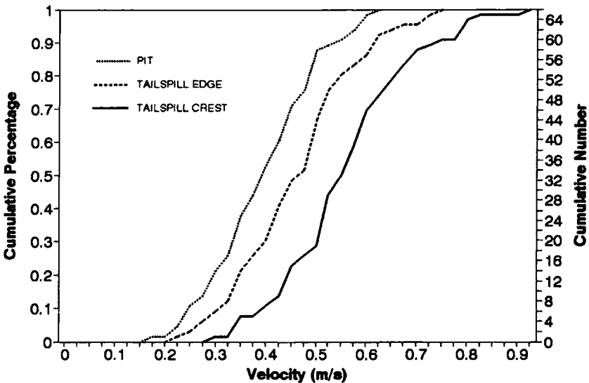
FIGURE 7.—Distribution of water velocities at three locations within Yellowstone cutthroat trout redds, Pine Creek, 1991.
