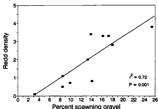
FIGURE 2.—Relationship between redd density (number/100 m 2 ) and percentage of the substrate consisting of potential spawning gravel in 11 reaches of Taylor Fork, 1992.
