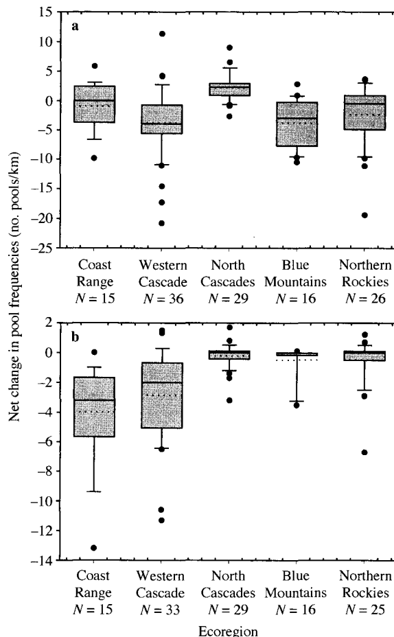
FIG. 6. Net change in the frequency of (a) large and (b) deep pools, by ecoregion. In the box plots, solid and dotted lines denote median and grand mean, respectively; boxes show 25th and 75th percentiles; whiskers show 10th and 90th percentiles; and circles denote outliers.
