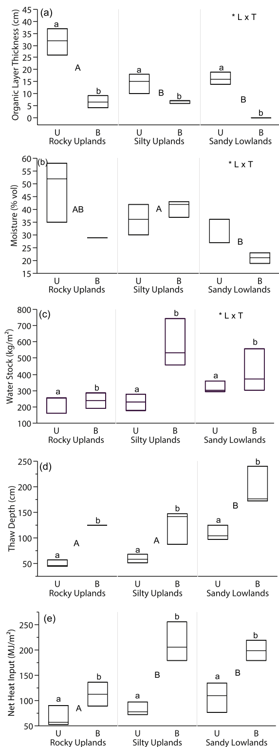
Figure 3. Box plots of surface organic layer thickness (a), volumetric soil moisture (b), water stock (c), thaw depth (d), and net seasonal heat input (e) across landscape types and treatments ( n = 17 ). Note, one outlier from a low-severity burn in the rocky uplands was excluded. Two-way ANOVAs and post hoc tests (Tukey HSD and student's t -tests) were conducted. Significant differences ( p < 0.05 ) between means are denoted by lowercase letters for treatment (unburned/burned) and uppercase letters for landscape type. Positioning of uppercase letters indicate the landscape-level means on the y-axes. Interactive effects of landscape and treatment ( *L \times T ) are displayed when significant.
