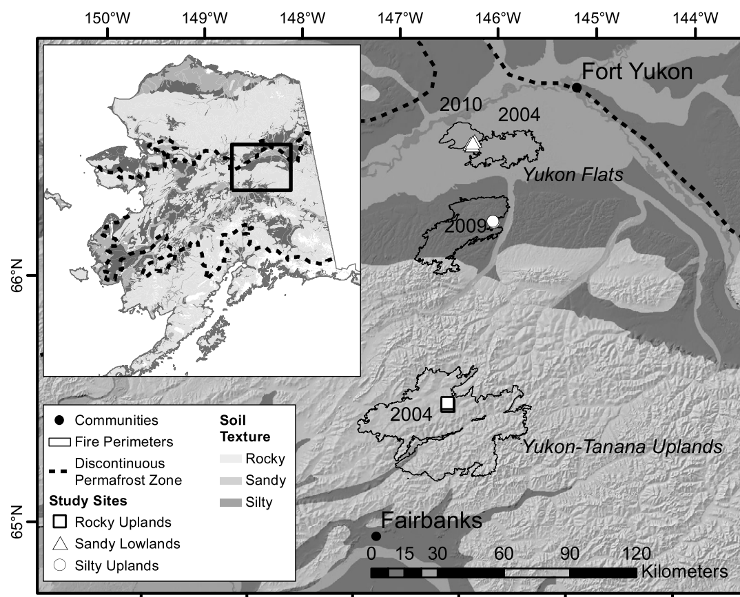
Figure 1. Topographic map of study area in interior Alaska. Dominant mineral soil textures are mapped with gray-scale symbology based on Karlstrom (1964) and Jorgenson et al (2008). The northern and southern boundaries of the discontinuous permafrost zone, from Jorgenson et al (2008), are represented with dashed lines. Study sites ( n = 18 ) are indicated by open squares (rocky uplands), triangles (sandy lowlands), and circles (silty uplands). Fire perimeters and year of burn are shown for the recent fires studied.
