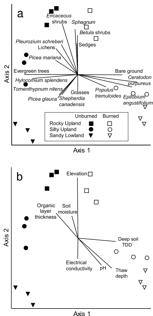
Figure 2. Nonmetric multidimensional scaling (NMDS) ordination of plant community structure and correlations with selected vegetation characteristics (a) and environmental characteristics (b). Points represent community structure at each site, and symbols differentiate between landscape types and treatment. Vectors show the direction and strength of the correlations. The ordination axes were rotated by the treatment variable (fire). The ordination axes represented 93% of the total variance in community structure, with 54% accounted for by Axis 1 and 39% by Axis 2.
