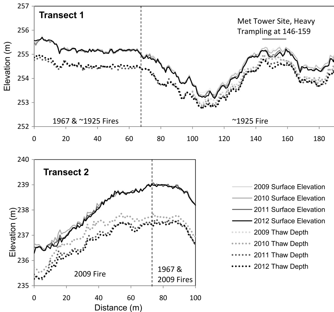
Figure 6. Cross-sectional profile of the elevation of the ground surface and permafrost surface along two transects in the silty uplands under different disturbance regimes from 2009 to 2012. Transect 1 burned around 1925 and a portion of it re-burned in 1967. Transect 2 burned in 2009, and a portion of it had previously burned in 1967. Note that the organic mat was compacted by human disturbance in Transect 1, with heavy trampling near a meteorological tower site.
