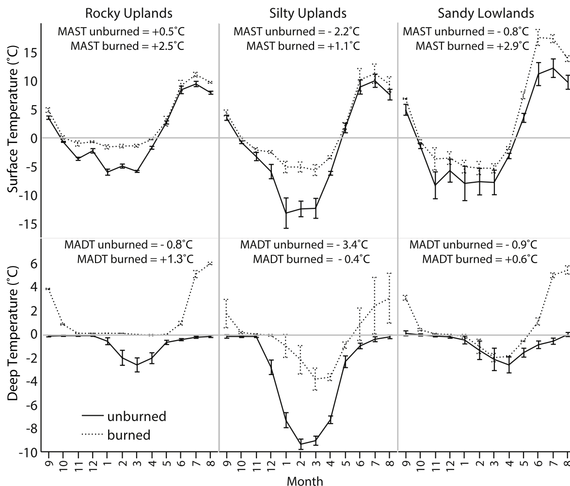
Figure 4. Monthly mean ( \pm SE) soil temperatures at the surface (5 cm) and at depth (100 cm) for unburned (solid line) and burned (dotted line) sites by landscape type from September 2011 to August 2012 ( n = 17 ). Note, one outlier from a low-severity burn in the rocky uplands was excluded. Mean annual surface temperatures (MAST) and mean annual deep temperatures (MADT) are displayed in text boxes.
