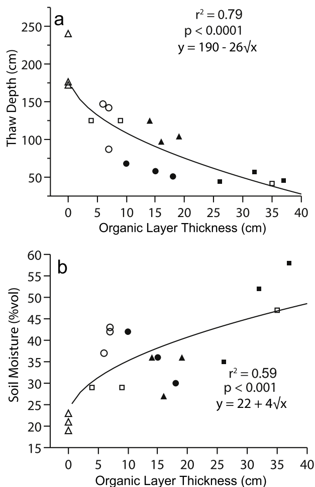
Figure 5. Relationships between surface organic thickness and thaw depth (a) and surface organic thickness and volumetric soil moisture (b) across all sites ( n = 18 ). Solid markers represent unburned sites, open markers represent burned sites. Triangles = sandy lowlands; circles = silty uplands; squares = rocky uplands.
