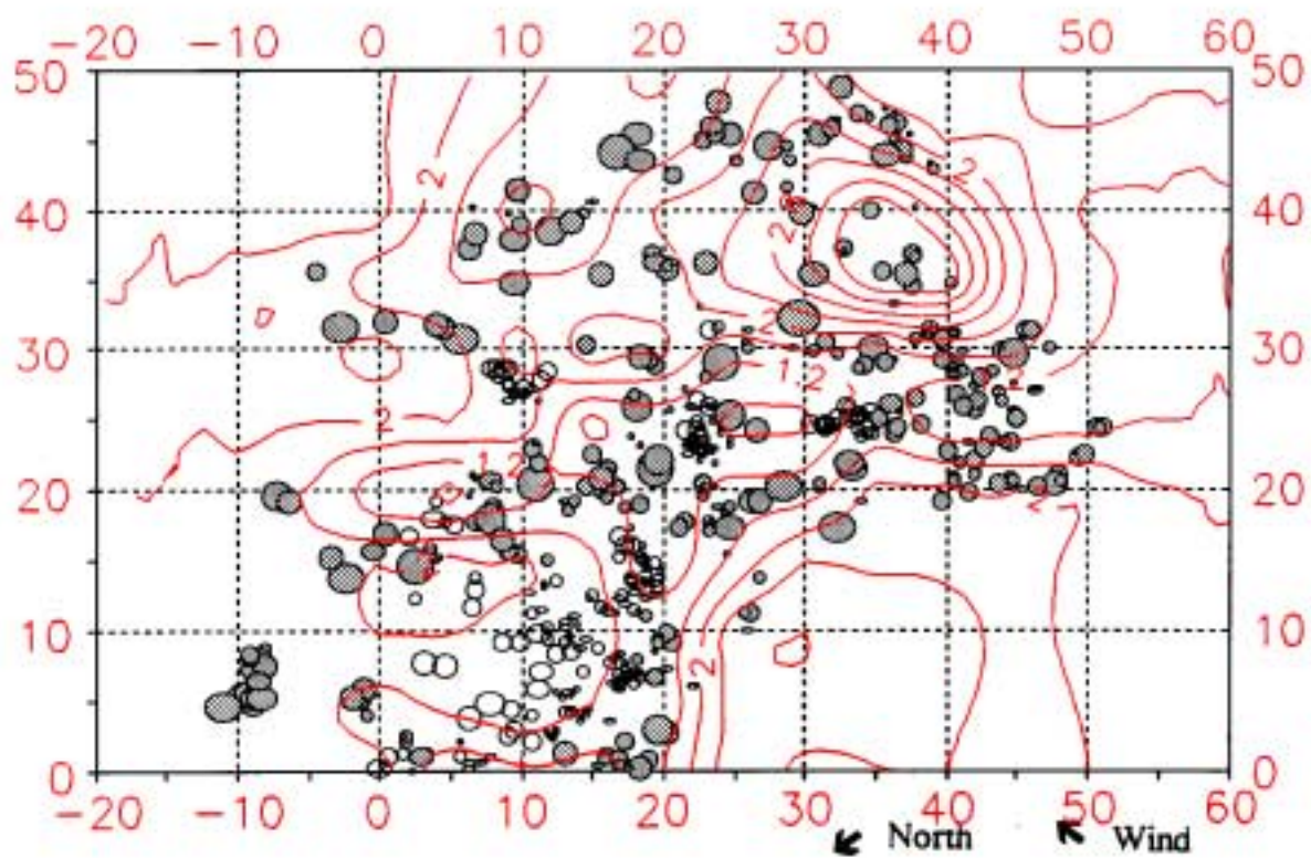
Figure 6.3. Map of snow depths at the ribbon plot, overlaid on a stem plot. Scale in meters; contour interval 0.4 m. Windward edge of plot is at right. In the stem map, circle diameter is proportional to DBH but has been exaggerated by 4x.
