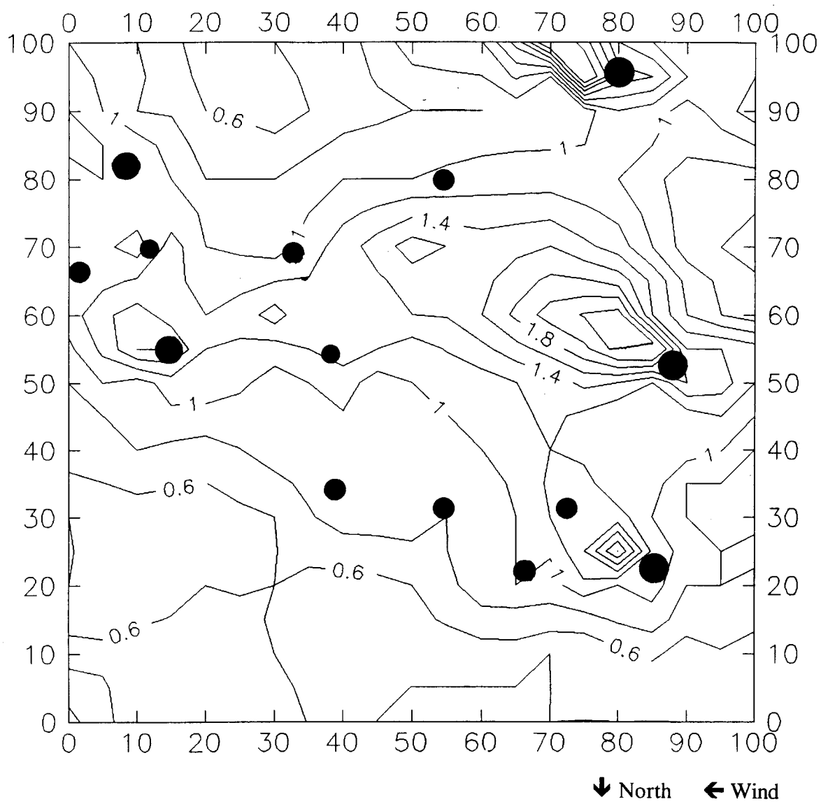
Figure 6.1. Map of snow depths at the clump plot. Large and small dots represent centers of the 5 large and 9 small clumps, respectively. Scale in meters; contour interval 0.2 m.
