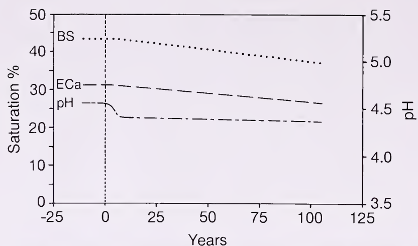
Figure 2.—Time course for soil base saturation (BS), exchangeable Ca (ECa), and pH from East Glacier simulations.
