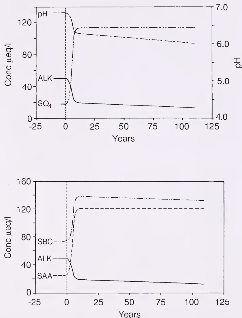
Figure 1.—Time course for East Glacier Lake outlet chemistry from baseline simulations. Precipitation SO 4 increased from 9.5 meq/m 3 to 60 meq/m 3 over a 5-year period starting with year one (precip pH approximately 4.3). Upper: ANC (ALK), pH, and SO 4 . Lower: ANC, sum of base cations (SBC), and sum of strong acid anions (SAA).
