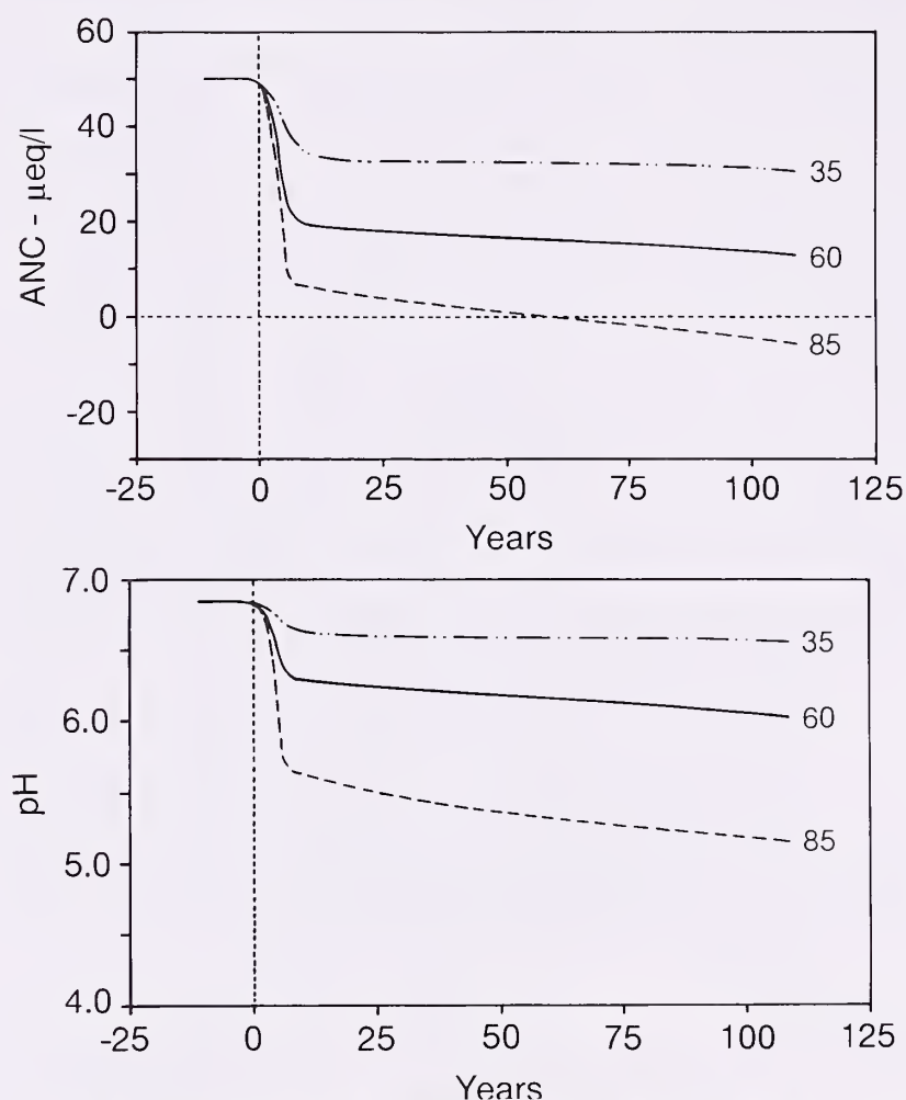
Figure 3.—Upper: ANC at East Glacier Lake outlet with wet deposition increasing to 35, 60, and 85 meq/m 3 over a 5-year period starting with year one. Lower: Time course for simulated pH.
