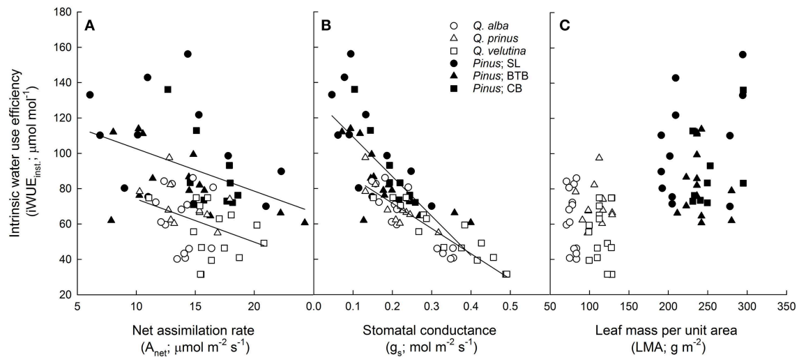
FIGURE 3 | Instantaneous intrinsic water use efficiency ( iWUE_{inst.} ; \mu\text{mol CO}_2 \text{ mol}^{-1} \text{ H}_2\text{O} ) vs. (A) net photosynthetic assimilation rate ( A_{net} ; \mu\text{mol CO}_2 \text{ m}^{-2} \text{ s}^{-1} ) for oaks ( y = -2.4x + 98.5 ; r^2 = 0.13 ) and pines ( y = -2.4x + 126.6 ; r^2 = 0.19 ), (B) stomatal conductance ( g_s ; \text{mol H}_2\text{O m}^{-2} \text{ s}^{-1} ) for oaks ( y = -143x + 100.3 ; r^2 = 0.79 ) and
