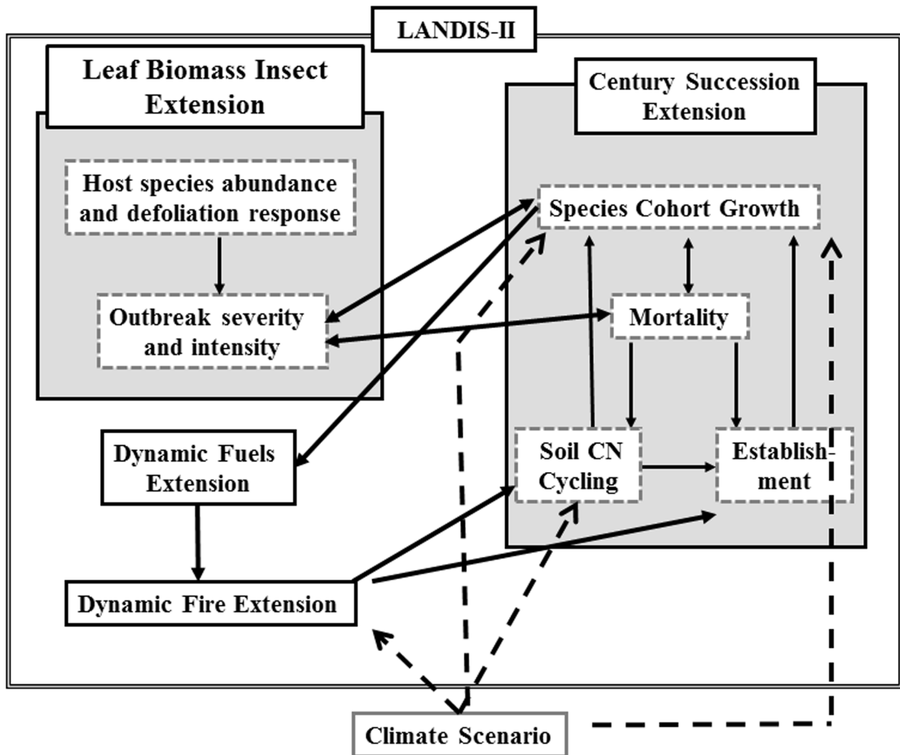
Figure 2. Conceptual diagram of LANDIS-II model. Arrows indicate interactions between model core, model extensions and climate scenarios. doi:10.1371/journal.pone.0102531.g002
