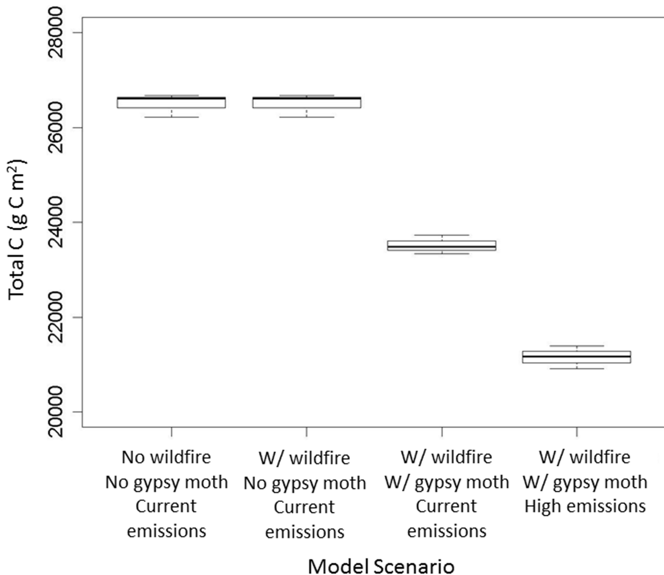
Figure 5. Total ecosystem carbon in four different model scenarios at simulation year 100. Scenarios 1–3 use baseline (current) climate, while the fourth uses the A2 (high emissions) scenario. 'w/GM' implies inclusion of gypsy moth outbreaks in the scenario. Confidence intervals represent standard errors based on 5 model replicates. Total carbon, was lowest when all three disturbances were operating on the landscape. Simulated wildfire had little impact on total C. doi:10.1371/journal.pone.0102531.g005
