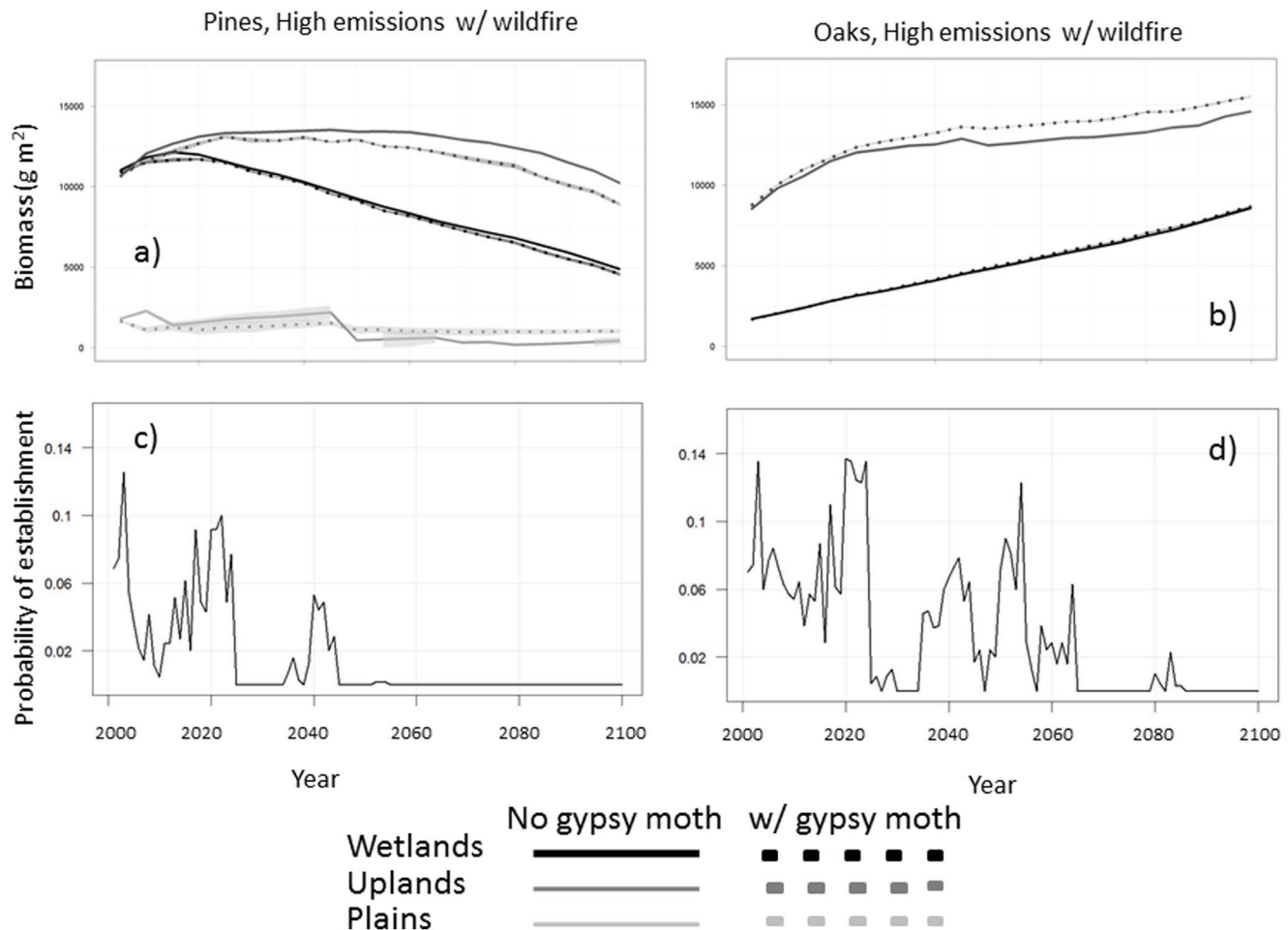
Figure 6. Aboveground biomass ( \text{g m}^{-2} ) for 'Oak' and 'Pine' functional groups over the course of the 100-year simulations. Plots a and b are comparisons of these groups under high emissions (A2) climate; Dotted lines represent scenarios with gypsy moth defoliation present. Ribbons surrounding each line are standard errors, based on five model replicates. Plots c and d show landscape probability of establishment for pine and oak functional groups under high emissions climate. doi:10.1371/journal.pone.0102531.g006
