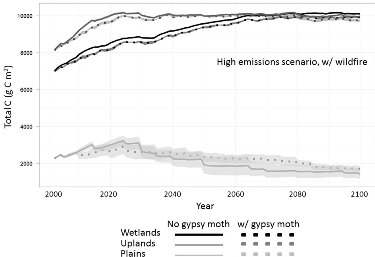
Figure 4. Total carbon under A2 (high emissions) climate scenario for all modeled ecoregion types. Reductions in the uplands and wetlands are a consequence of gypsy moth defoliation (dotted lines). Total carbon in the plains, represented in light grey, did not significantly change over the 100-year scenario.
