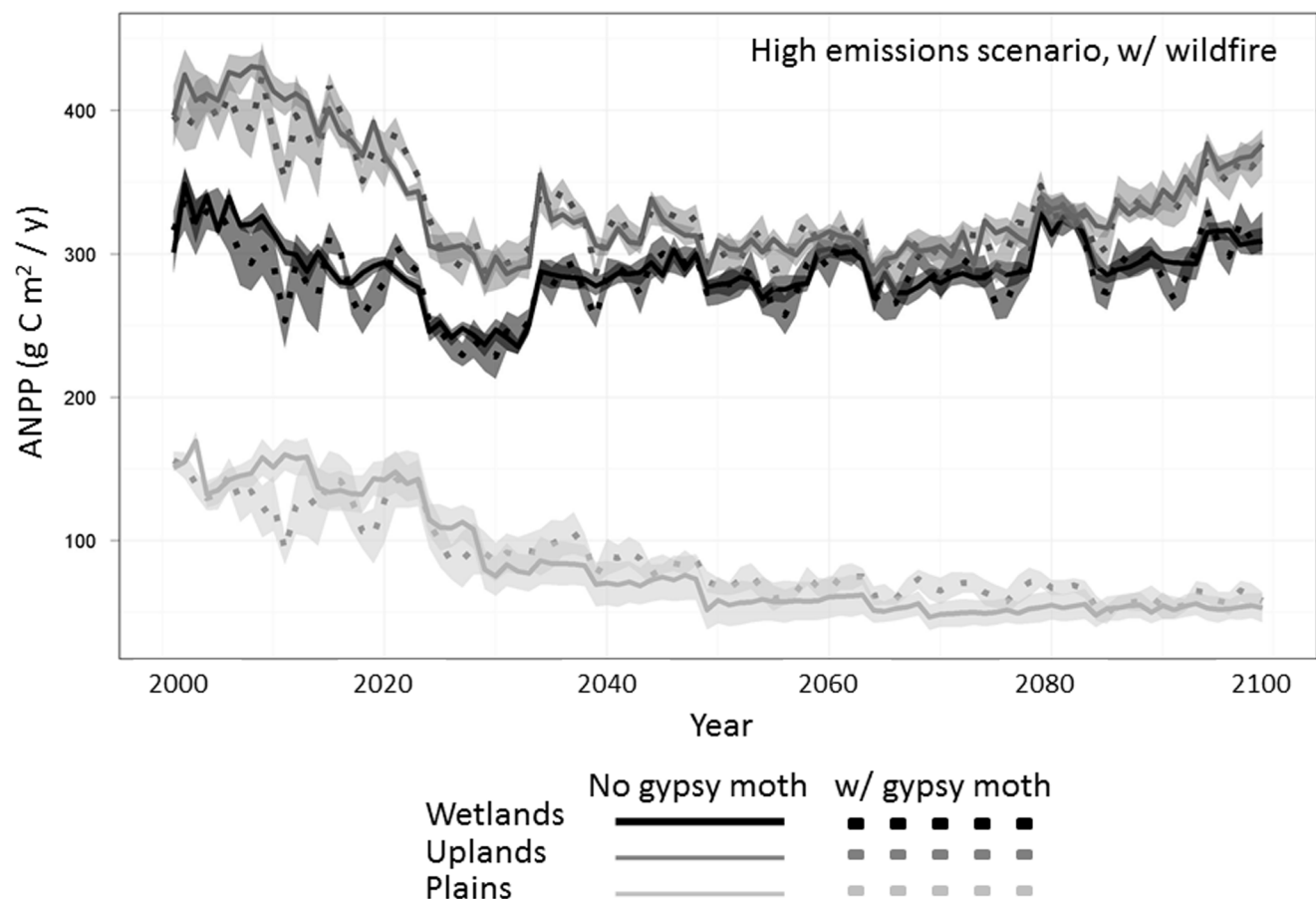
Figure 3. Aboveground net primary production (ANPP) in the three modeled ecoregion types under A2 (high emissions) climate scenario. Scenarios which included gypsy moth defoliation are seen in the dotted lines. Ribbons surrounding each line represent the standard error, based on five model replicates.
