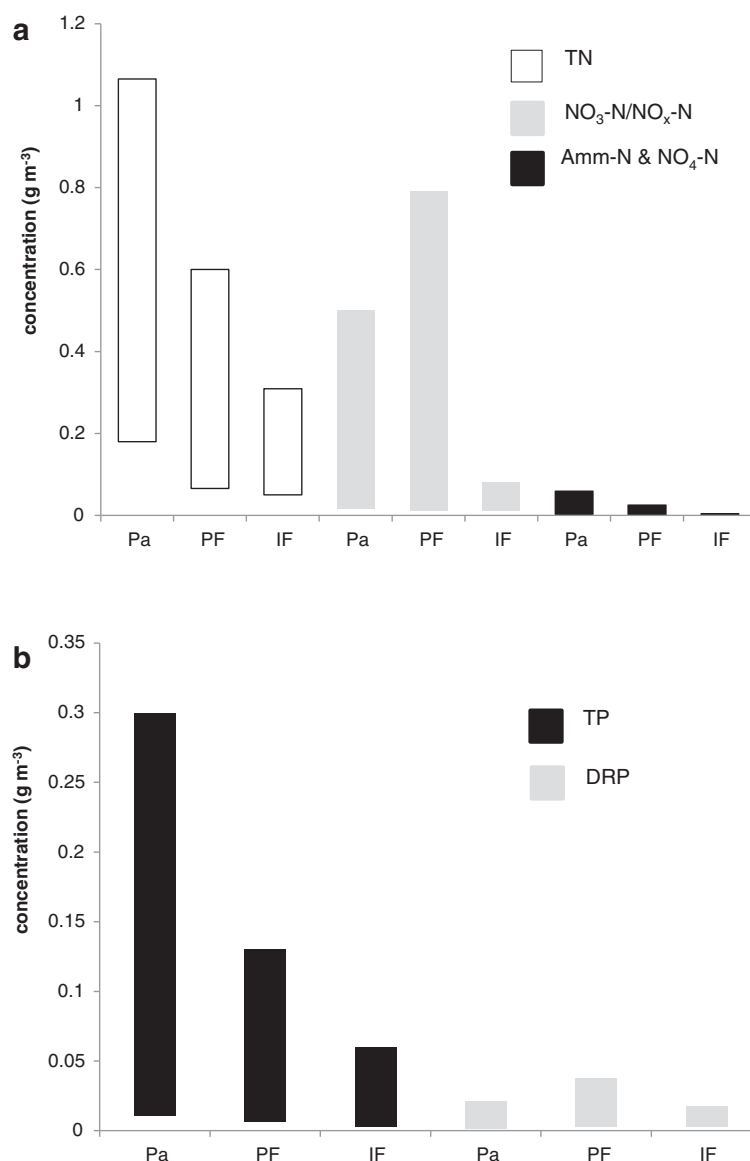
Figure 4 Range of TN, NO 3 -N (a), TP and DRP (b) mean and median concentrations recorded in pasture (Pa) (n = 33), mature planted forest (PF) (n = 53) and indigenous forest (IF) (n = 35) streams. NO x -N values have been aggregated with NO 3 -N as nitrite is rapidly oxidised to nitrate and typically comprises a small portion of oxidised-N. Similarly Amm-N values have been aggregated with NH 4 -N values as NH 3 -N comprises a small component of Amm-N. Mean and median concentrations derived from tables and text or estimated from figures in references (Fahey and Stansfield 2006; Friberg et al. 1997; Macaskill et al. 1997; Matheson et al. 2011; Parkyn et al. 2006; Thompson and Townsend 2004b; Townsend et al. 1997; Young et al. 2005). The anomaly of a wider range of NO 3 -N/NO x -N concentrations than TN concentrations in planted forest streams (Figure 4a) was influenced by Fahey & Stansfield's (2006) Hawke's Bay study and probably due to the lower sampling intensity of TN, capturing a smaller range of concentrations compared with NO 3 -N (sample size for NO 3 -N and TN, 62-64 and 3-4 respectively).
