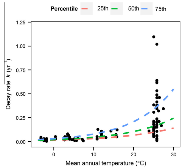
Fig. 5. Decay rates ( k ) reported for downed woody debris density and/or mass at three corresponding percentiles. Parameter estimates can be found in Table 4. For a list of studies included in this figure, see Supplemental Material 2.
