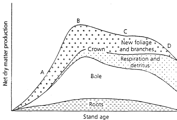
Fig. 5.4 Generalized pattern of net primary productivity assimilation into principal tree components of a forest stand. Major phases are: A, rapid increases in assimilation rates as crowns expand when stand is below leaf area carrying capacity; B, peak productivity at crown closure; C, period of maturity — leaf area is fixed and an increasing proportion of gross assimilation is used as maintenance respiration; D, rapid decline as stand senesces from natural causes. (Modified from Waring & Schlesinger 1985.)
