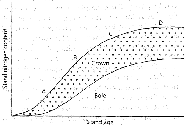
Fig. 5.5 Generalized pattern of nitrogen accumulation in above-ground biomass of a developing stand—derived from Fig. 5.4.
