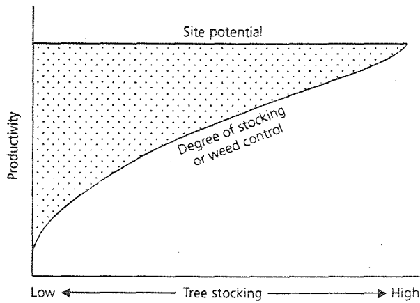
Fig. 5.2 Relationship between degree of stocking (or weed control) and the potential productivity inherent to a site. Improved stocking or weed control captures a greater proportion of the site's inherent potential.
