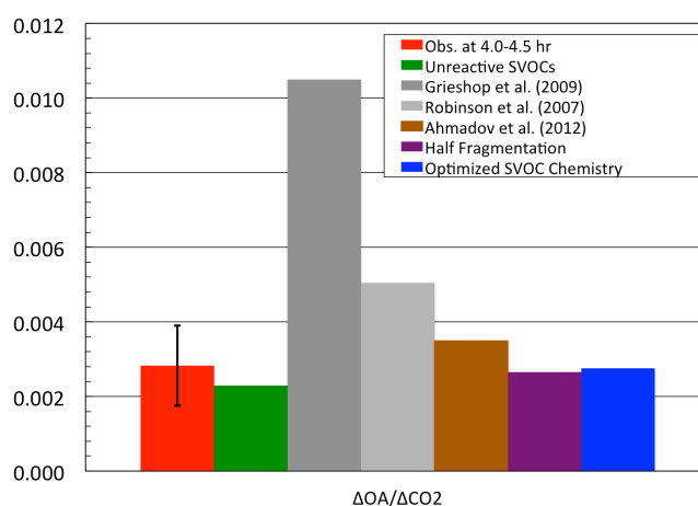
Figure 9. Enhancement ratio (EnR; \text{g g}^{-1} ) of organic aerosol (OA) to \text{CO}_2 after 4 to 4.5 h of smoke aging. The error bars on the observed values are based on the 36% uncertainty in the AMS observations of OA. All model results assume the best-estimate dilution rate and the photolysis rates corresponding to the middle of the plume (solid black line in Fig. 4).
