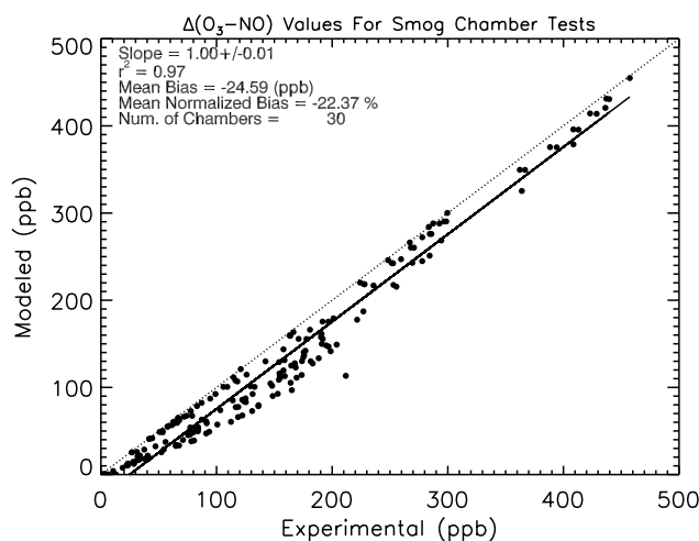
Figure 1. ASP calculated hourly values of \Delta([\text{O}_3] - [\text{NO}]) \equiv ([\text{O}_3]_{\text{final}} - [\text{NO}]_{\text{final}}) - ([\text{O}_3]_{\text{initial}} - [\text{NO}]_{\text{initial}}) vs. the values measured in the EPA chamber of Carter et al. (2005) for 30 “full surrogate” experiments. Note that all time points for the 30 chamber experiments are plotted, not just the final values.
