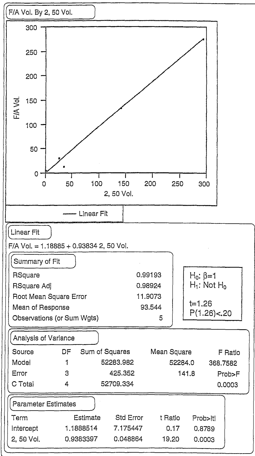
Figure 3. The volume estimated with 2, 50 meter line segments was regressed against the actual volume on each \frac{1}{4} hectare fixed-area plot, with OLS. The relationship was significant and the coefficient of the independent variable was equal to one. The intercept coefficient was not significant. OLS results indicated that the line transect method accurately estimated large down debris on \frac{1}{4} hectare plots.
