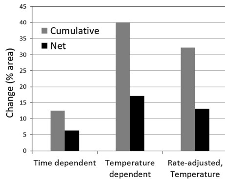
Fig 1 Projected cumulative and net changes in overall area by ecosystem changes from 2010 to 2100 within the ARCN study area
