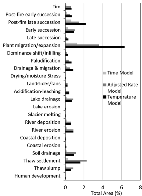
Fig. 4 Changes in cumulative area (%) during the final 2070–2100 period caused by 23 biophysical 4 drivers used in the three state-transition models
