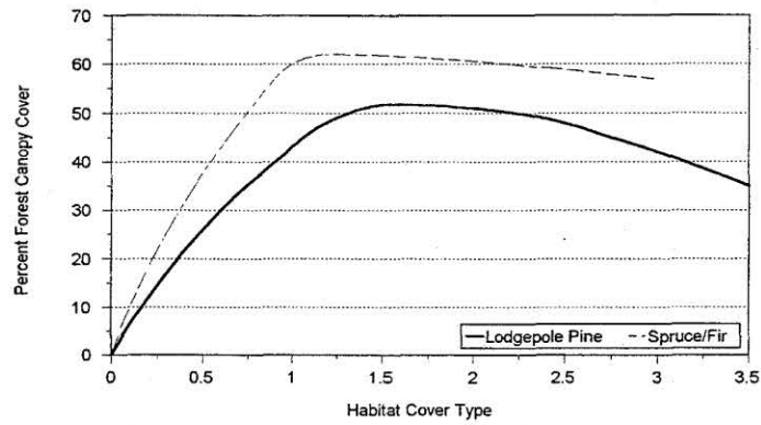
Figure 3. Relationship between percent canopy measured with a photcanopyometer and the habitat cover type index for lodgepole pine and spruce/fir stands on the Tenderfoot Creek Experimental Forest.
