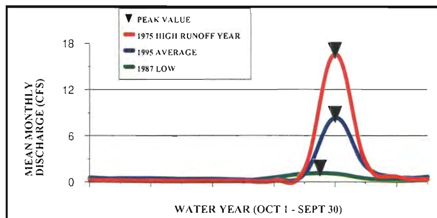
FIGURE III-3 SUN CREEK HYDROGRAPHS NATURAL RANGE OF VARIATION FORESTED CONDITIONS
