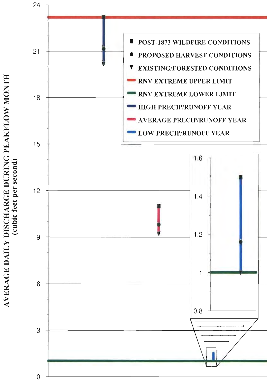
FIGURE III-4 SUN CREEK RANGE OF VARIATION IN PEAKFLOW
