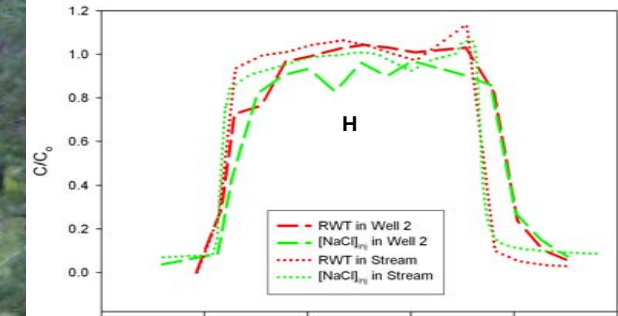
Concentration / Average Concentration During Injection
