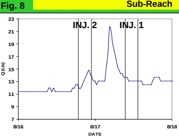
Fig. 8: Several small storms passed through the watershed over the injection period. The changing discharge may have effected our ability to estimate solute transport parameters, especially during the first injection.
