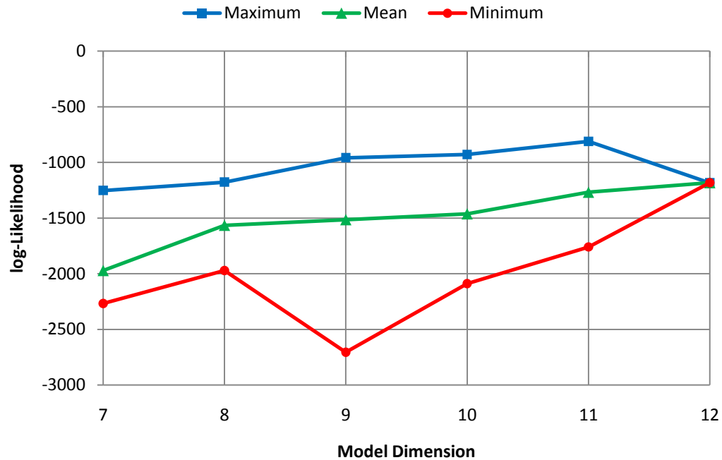
Figure 5.1: Calibration results, showing maximum, mean and minimum log-likelihood value for each model dimension.
