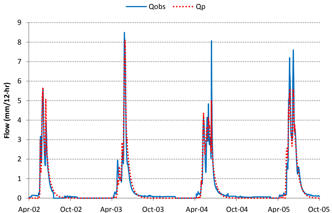
Figure 5.6: Hydrograph simulation for the PDMsdE_TRn model structure and the calibration data set.
