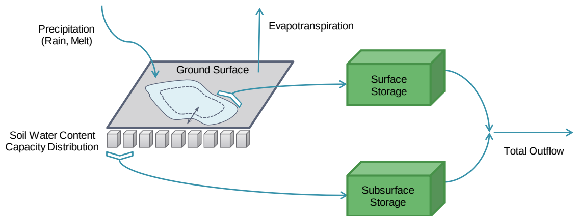
Figure 4.5: A schematic representation of the TOPMODEL soil moisture accounting and runoff routing component.
