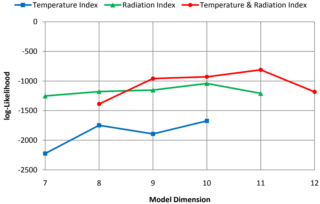
Figure 5.3: Calibration results grouped by the snowmelt accounting component. Snowmelt components utilizing net radiation data far outperform the simple temperature index approach across all model dimensions.
