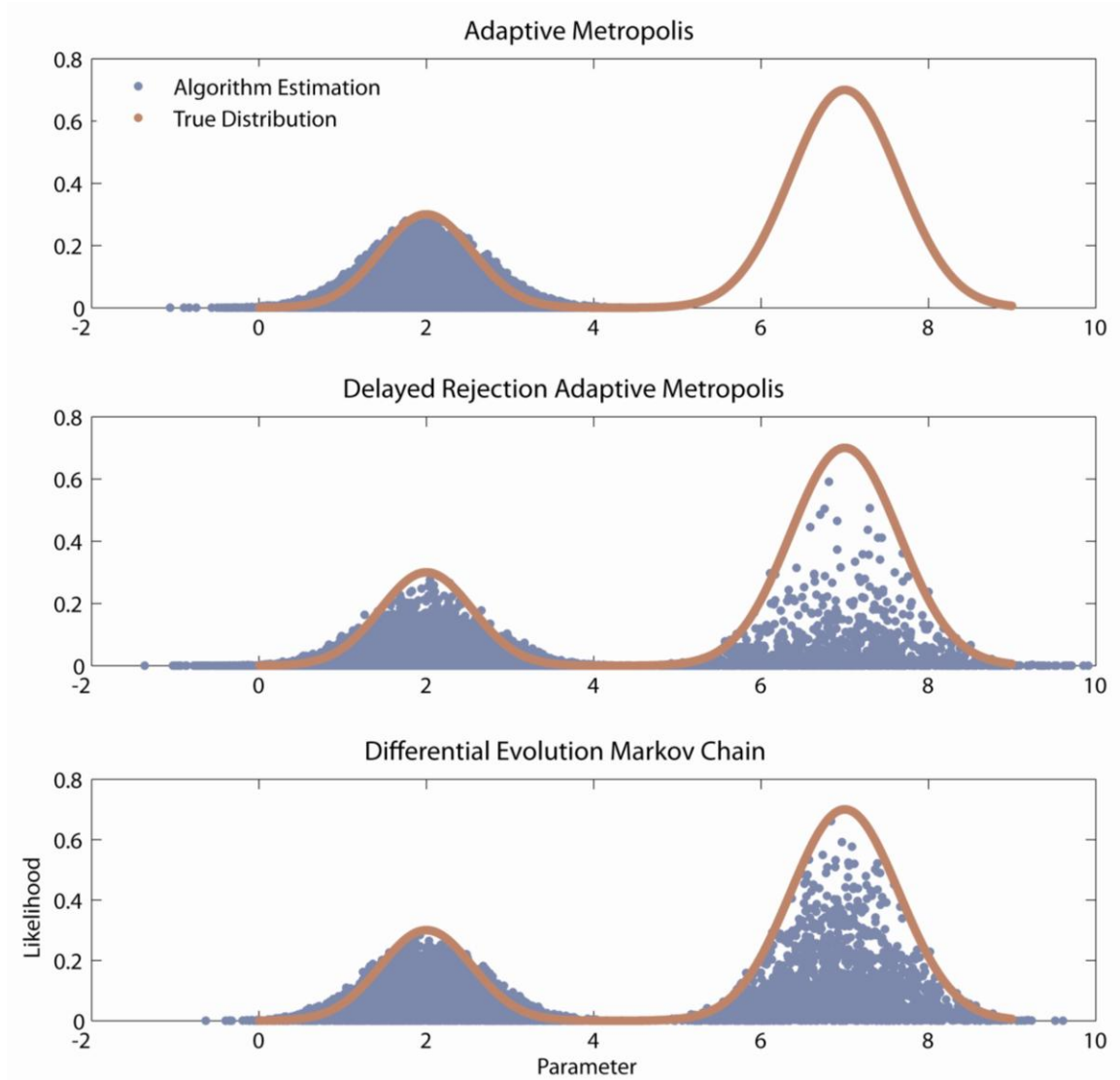
Figure 3.2: Comparison of parameter estimation between the AM, DRAM and DE-MC algorithms for 50,000 iterations and one parameter for a five-dimensional Gaussian mixture. Values shown in blue were sampled in 5-D space and were projected into 1-D space. The exploration of the parameter surface is weakest in the AM algorithm, with only one mode sampled, while the DRAM and DE-MC algorithms manage to sample each mode.
