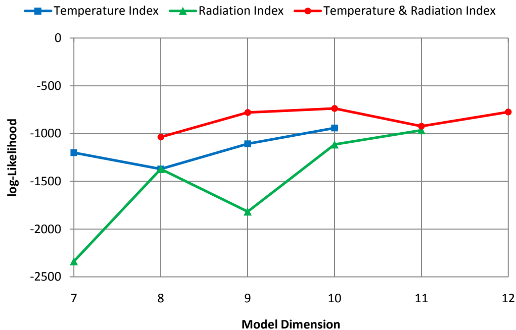
Figure 5.10: Validation results grouped by the snowmelt accounting component.
