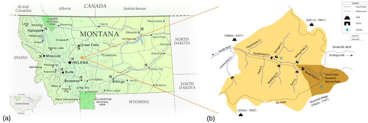
Figure 4.1: Tenderfoot Creek Experimental Forest; (a) location and (b) instrumentation. Adapted from Jencso et al. (2008, In Review) and < http://www.fs.fed.us/rm/ecology/demo/tenderfoot/ >.
