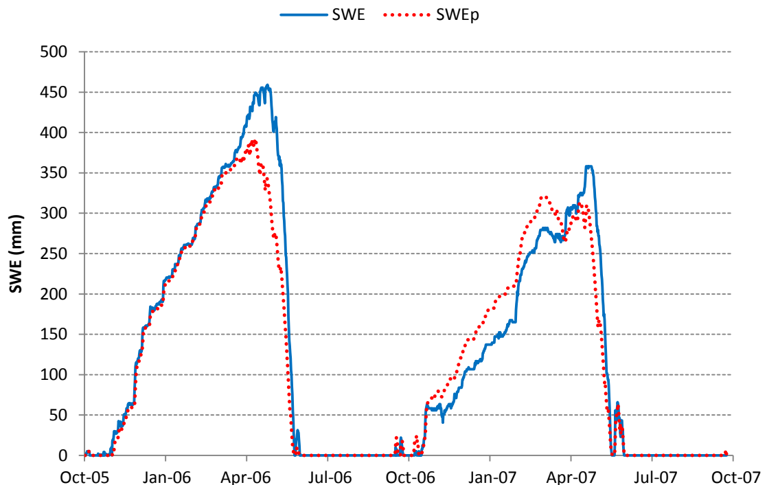
Figure 5.20: Snow water equivalents simulation for the PDMsdE_TRn model structure and the validation data set.
