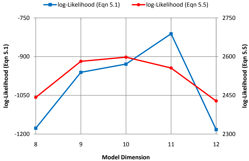
Figure 5.12: Likelihood function comparison for the best Probability Distributed Model based structure at each dimension. A similar pattern exists across the differing likelihood functions relating performance and complexity.
