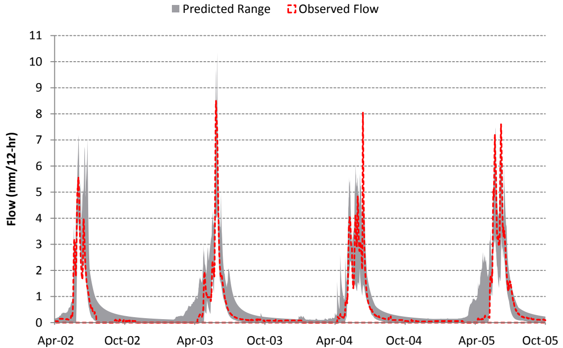
Figure 5.13: Range of predictions on the calibration data set from the collection of model structures investigated.
