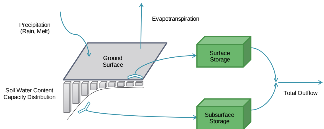
Figure 3.3: The Probability Distributed Model with snowmelt as an additional precipitation input.
