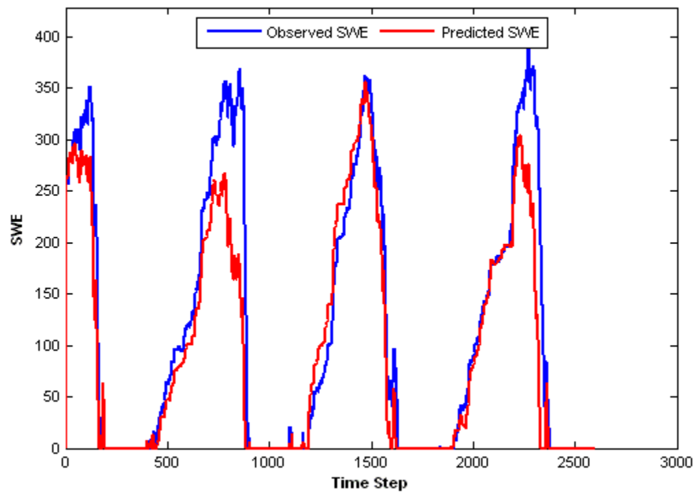
PLOT: Simulation Snow Water Equivalents
