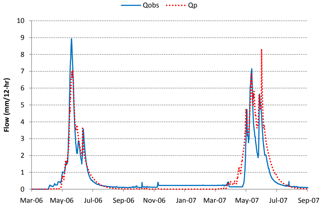
Figure 5.7: Hydrograph simulation for the PDMsdE_TRn model structure and the validation data set.
