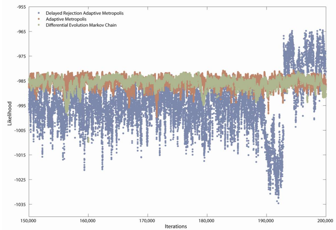
Figure 3.4: Comparison of AM, DRAM and DE-MC parameter searches, started from a point of known low posterior density. The AM and DE-MC falsely converge to a local optimum, while the DRAM locates a region of higher posterior density.
