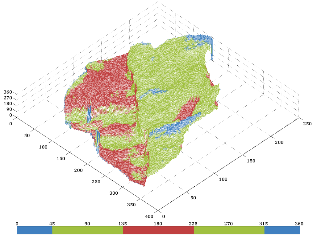
Figure 4.6: Semi-distribution of precipitation by aspect.
