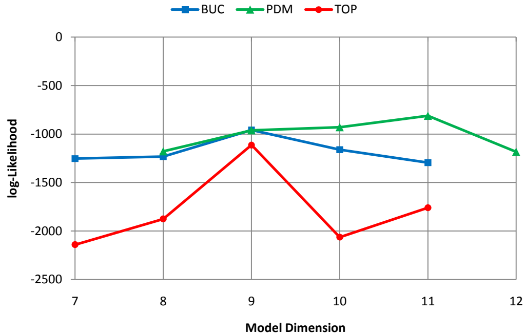
Figure 5.2: Calibration results grouped by the soil moisture accounting and runoff routing component. The PDM component results in the best performance at each dimension.
