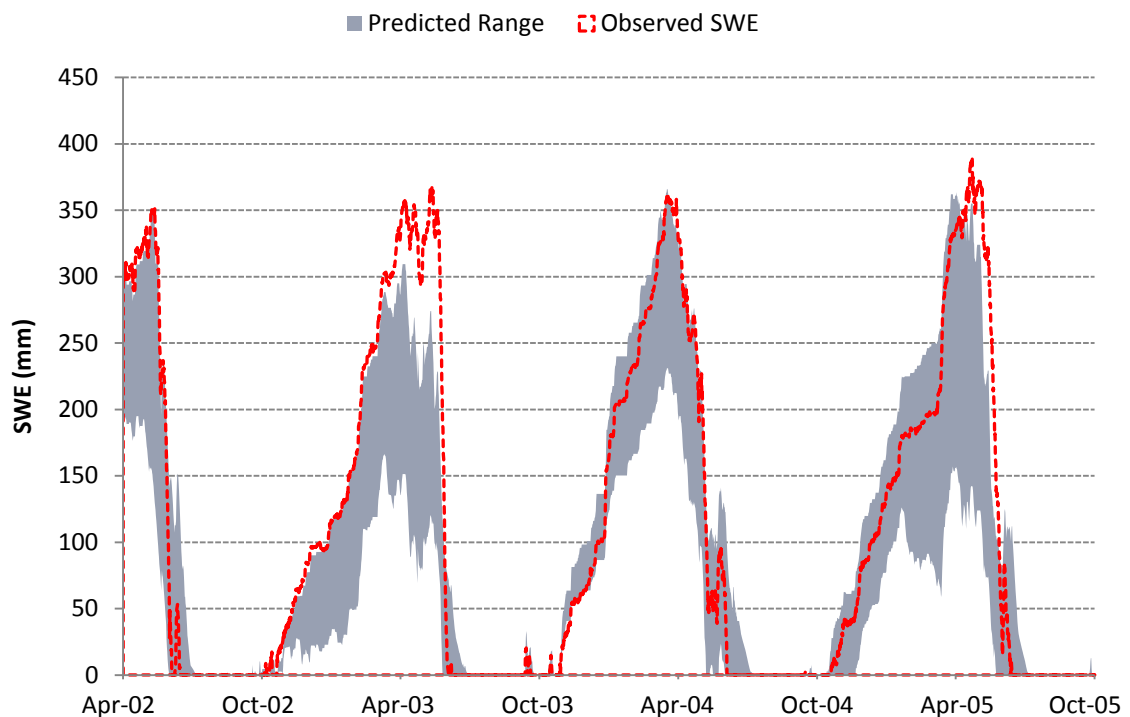
Figure 5.21: Snow water equivalents ensemble simulations for each model structure and the calibration data set.
