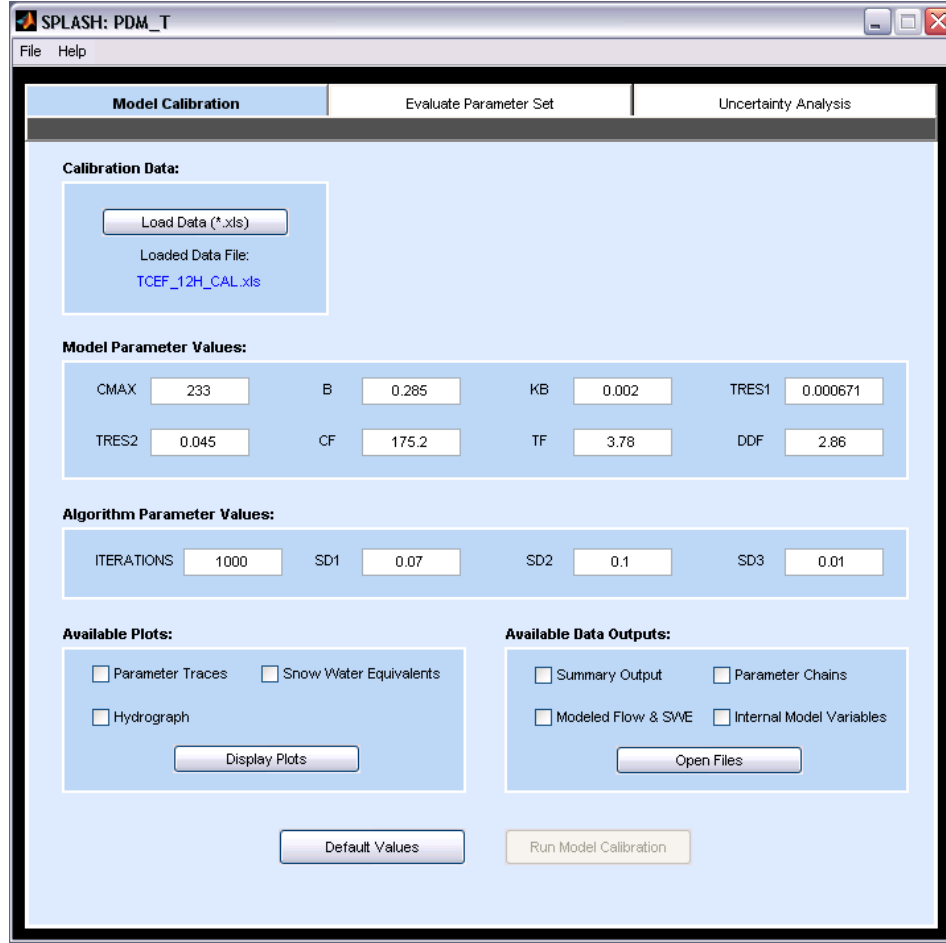
Figure 6.3: Model calibration tab within SPLASH.
