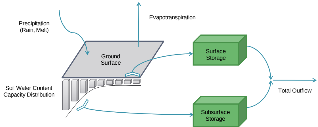
Figure 4.4: A schematic representation of the Probability Distributed Model soil moisture accounting and runoff routing component.
