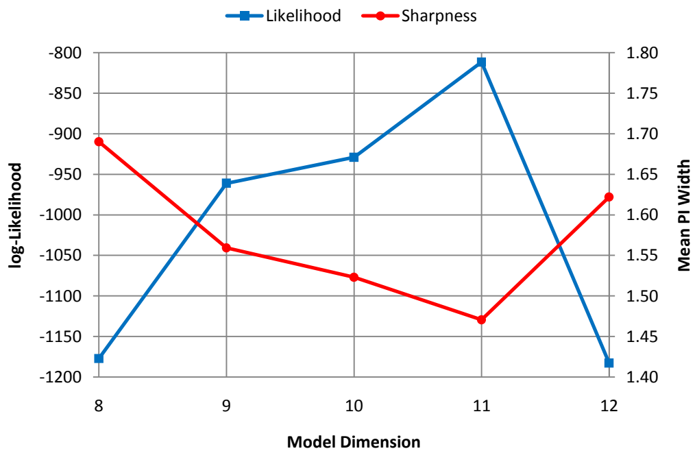
Figure 5.16: Comparison of sharpness and log-likelihood versus model dimension. There is a general inverse relationship seen between sharpness and log-likelihood, suggesting that the sharpest models are the best performing.
