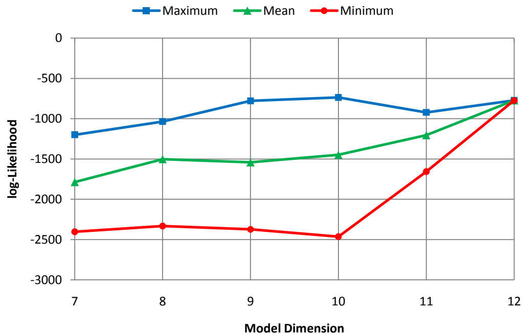
Figure 5.8: Validation results grouped by maximum, mean and minimum log-likelihood value for each model dimension. On average, there is an increase in predictive performance with an increase in complexity, similar to the calibration period.
