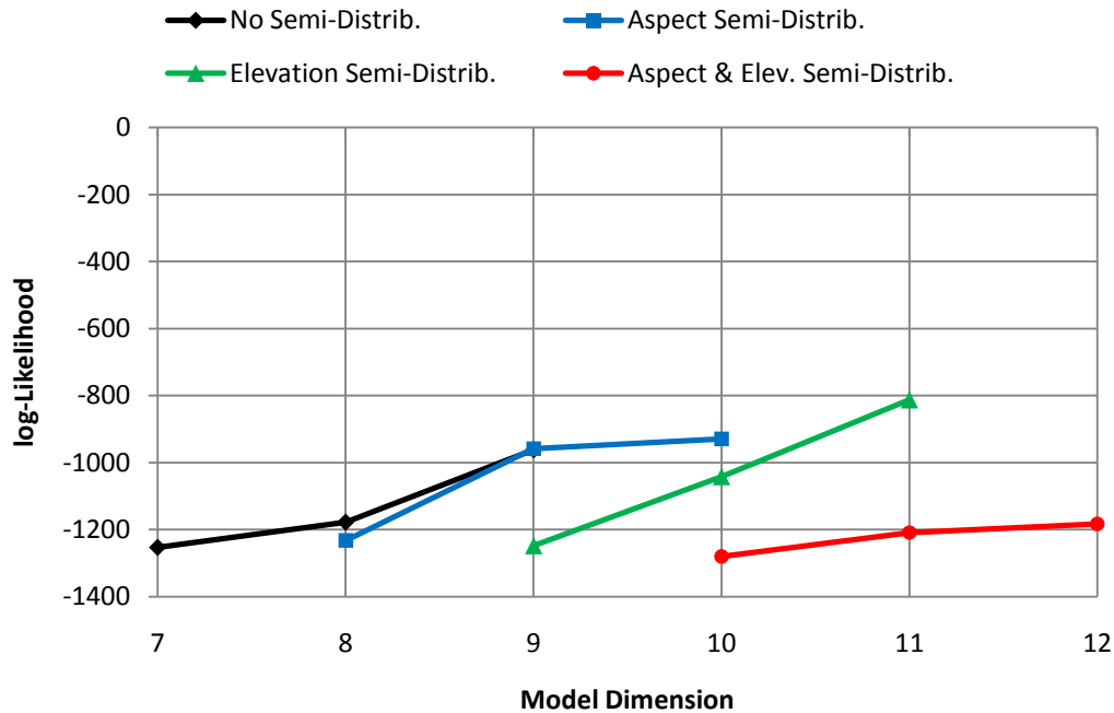
Figure 5.4: Calibration results grouped by the precipitation semi-distribution component. This comparison indicates the precipitation semi-distribution approaches provide little to the model aside from additional flexibility.
