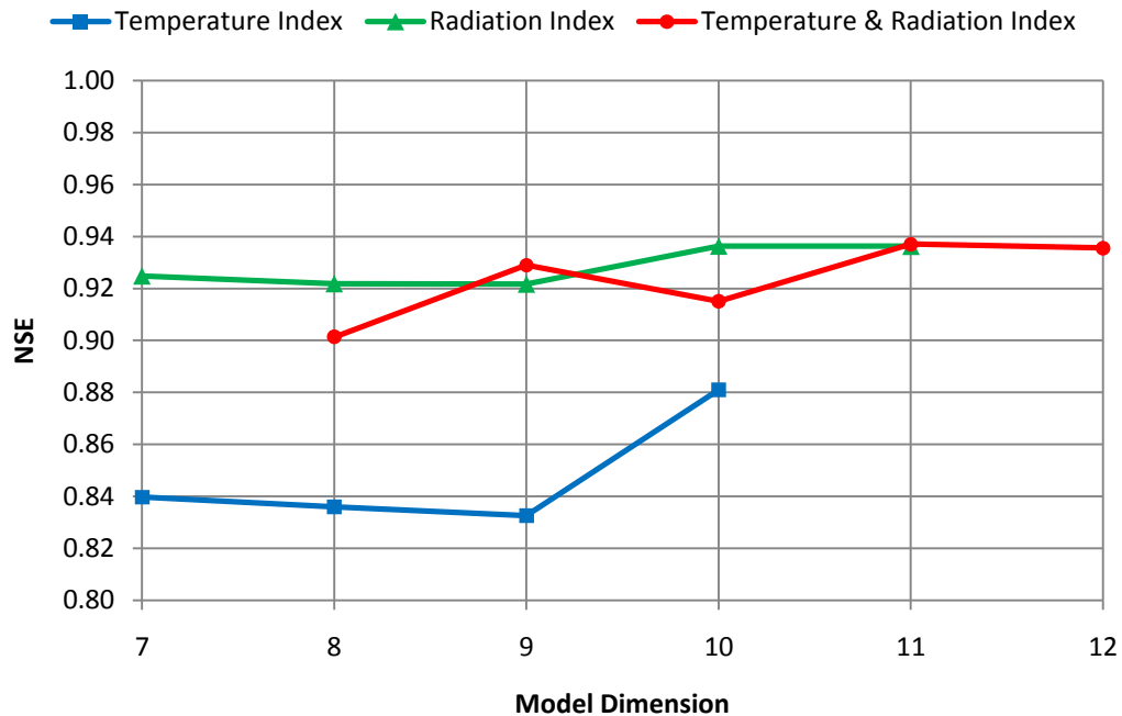
Figure 5.18: Snow water equivalents simulation results grouped by snowmelt accounting component for each model dimension over the calibration period. The temperature index approach is shown to be the least effective snowmelt accounting method over this period.
