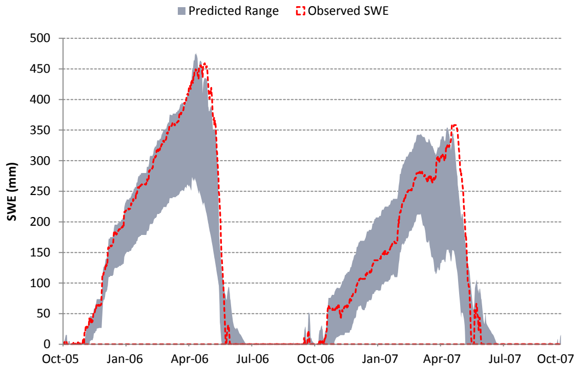
Figure 5.22: Snow water equivalents ensemble simulations for each model structure and the validation data set.
