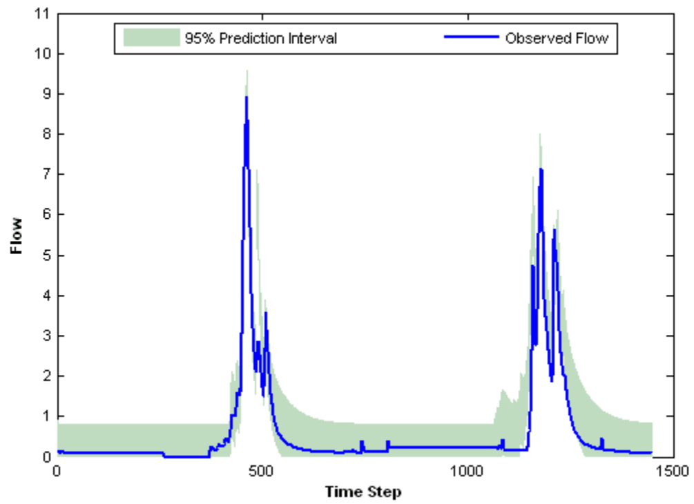
PLOT: 95% Prediction Interval Hydrograph
