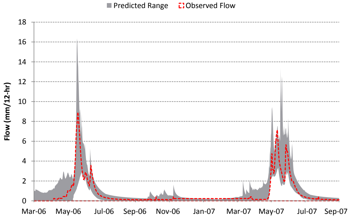
Figure 5.14: Range of predictions on the validation data set from the collection of model structures investigated.
