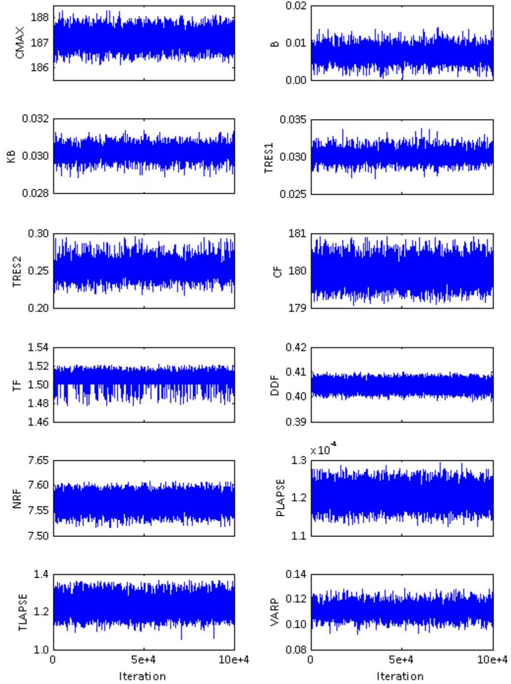
Figure 5.5: Parameter traces from the calibration of the PDMsdE_TRn model structure. Each parameter for this structure was shown to have converged based on visual inspection. Units are as previously defined.
