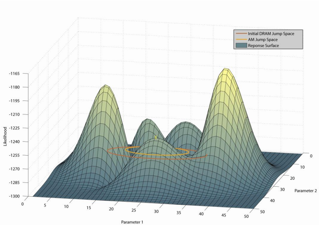
Figure 3.1: Hypothetical parameter surface illustrating the ability of the AM and DRAM algorithms to explore the parameter surface. Rings represent distance from the current location an algorithm can explore.
