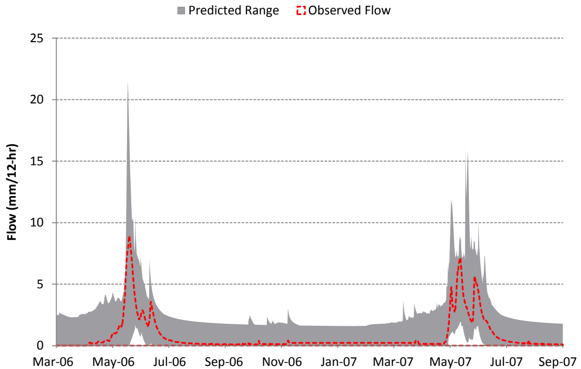
Figure 5.17: Range of predictions on the 95% prediction intervals over the validation data set from the collection of model structures investigated.
