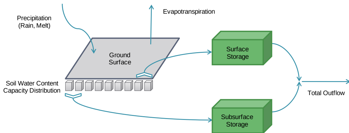
Figure 4.3: A schematic representation of the bucket model soil moisture accounting and runoff routing component.
