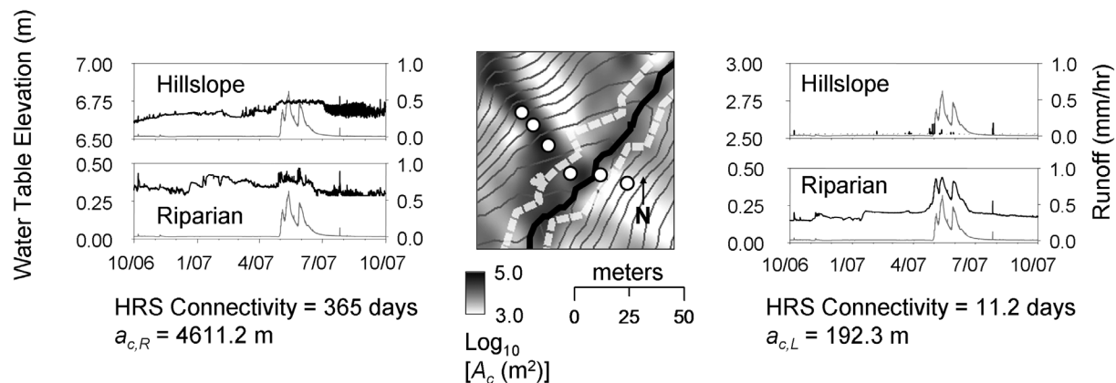
Figure 9. Stringer Creek transect 5 east and west hillslope and riparian water table (black lines, elevation is relative to local datum) and runoff (gray lines) dynamics. Specific area for each side of the transect and the total time of hillslope-riparian-stream connectivity (days) during the 2007 water year are listed below each time series. The map in the middle depicts the transects contributing area A_c (dark shading corresponds to high values of A_c and light shading indicates low values of A_c ), contour lines (gray lines), riparian zone extents (white dashed lines), well locations (white circles), and stream position (black line).
