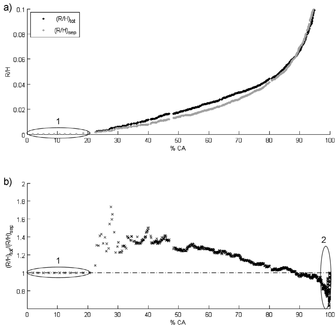
Figure 7. Comparison of riparian-hillslope ratios ( R/H ) calculated based on total and side-separated values. (a) Cumulative area-weighted distributions of riparian-hillslope ratios (R/H)_{sep} and (R/H)_{tot} . (b) Ratios of the above distribution functions. Areas labeled 1 and 2 are explained in the text.
