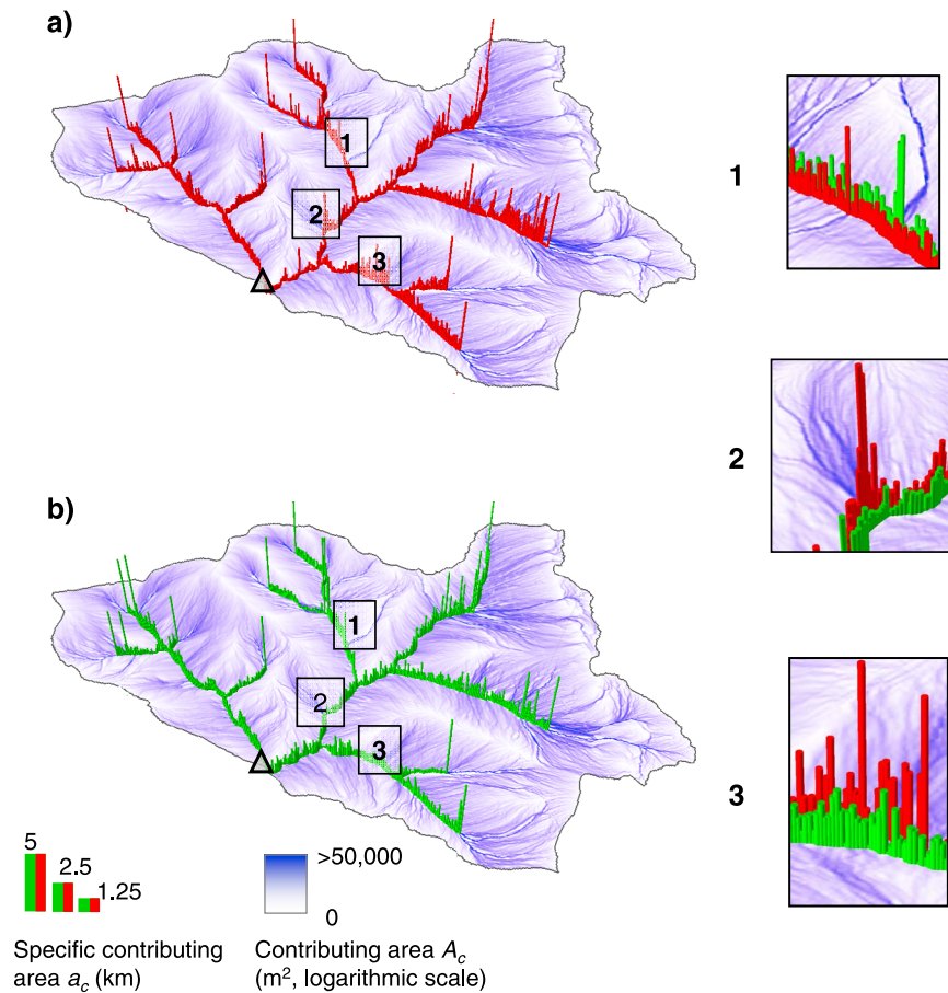
Figure 5. Spatial representation of contributing area A_c (blue-shaded flow lines) and side-separated specific contributing area values a_c from left (green bars) and right (red bars) stream sides. (a) Illustrates the specific contribution area values from right stream sides, a_{c,R} , while (b) shows the contributions from left stream sides, a_{c,L} . Insets (1, 2, and 3) represent close-up views of selected stream locations in the catchment. Triangles mark the outlet of the Tenderfoot Creek experimental catchment.
