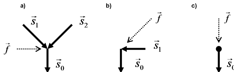
Figure 2. Different configurations of flow lines \vec{f} (dotted arrows) and stream vectors \vec{s}_i , i \geq 0 (plain arrows). (a) Stream junction: In this example, the flow line \vec{f} is located on the right stream side because it is on the right side relative to all stream vectors \vec{s}_i . (b) Sharp stream bend: In this example \vec{f} is on the left side relative to \vec{s}_0 and on the right side relative to \vec{s}_1 and therefore on the outer side of the bend. Since the cross product \vec{s}_1 \times \vec{s}_2 has a positive z component the inner bend must be located on the left stream side and \vec{f} , hence, is on the right stream side. (c) Channel head: In this example the orientation of the flow line \vec{f} relative to \vec{s}_0 is not definable.
