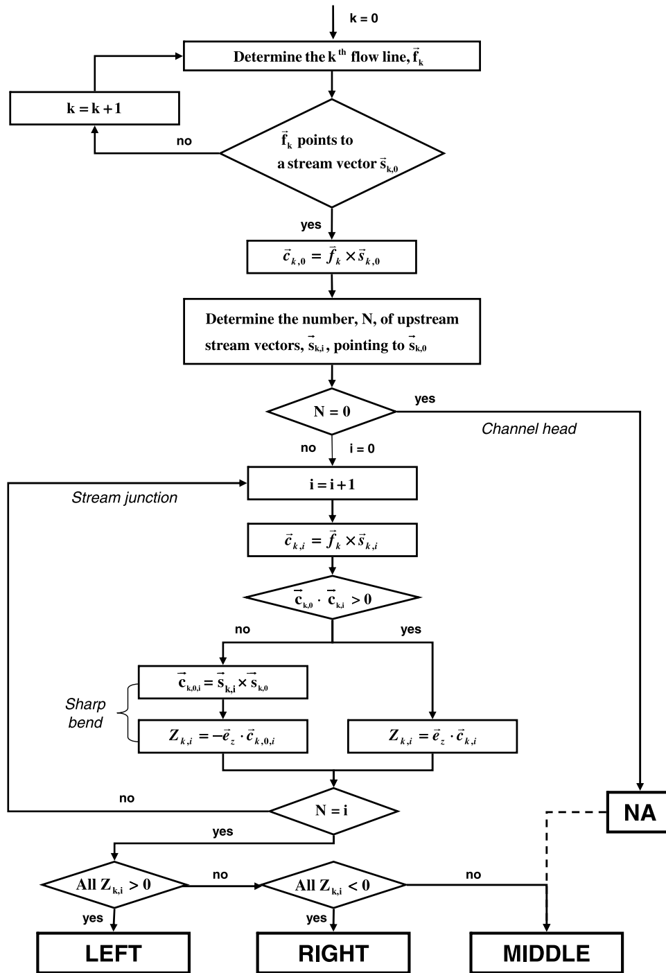
Figure 3. Flowchart illustrating the determination of a hillslope position. Symbols are defined in the notations list.
