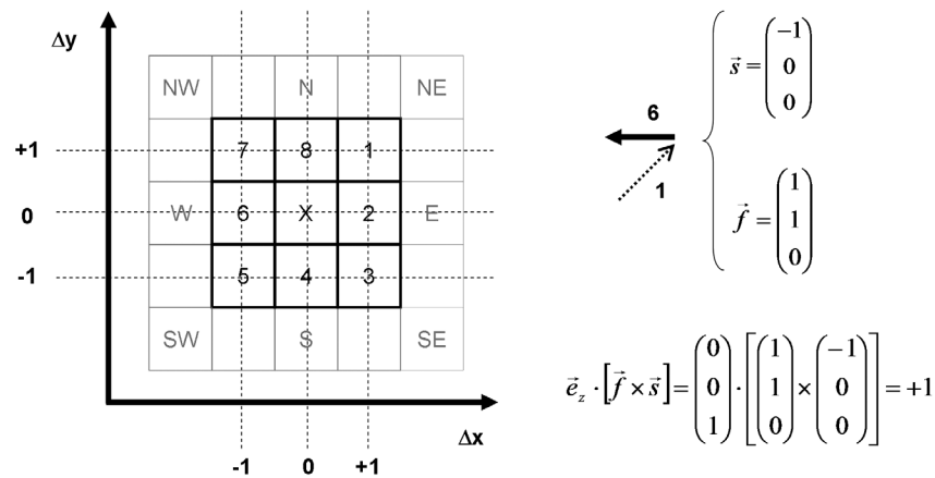
Figure 1. Stream flow direction grid. Directions relative to center grid cell X are coded from 1 to 8 clockwise from northeast (NE) to north (N). The corresponding vector notation is illustrated for flow line vector \vec{f} in direction 1 (dotted arrow) and for streamflow vector \vec{s} in direction 6 (plain arrow). Calculating the cross product \vec{f} \times \vec{s} reveals a positive z component and therefore flow line vector \vec{f} is located on the left side relative to stream vector \vec{s} .
