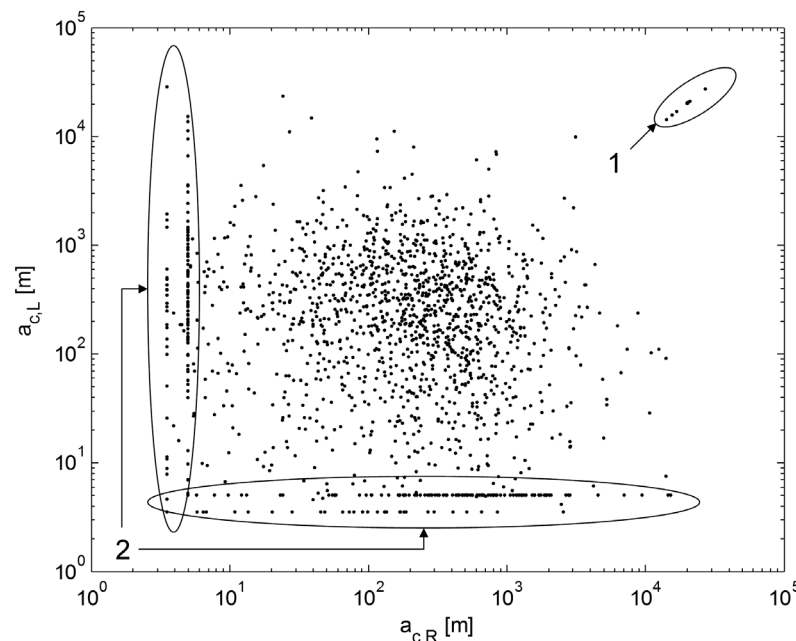
Figure 6. Scatter plot of right specific lateral contributing areas ( a_{c,R} ) versus their counterparts on the left stream side ( a_{c,L} ) along the stream network of the 23 km 2 Tenderfoot Creek Experimental Forest catchment. Areas labeled 1 and 2 are explained in the text.
