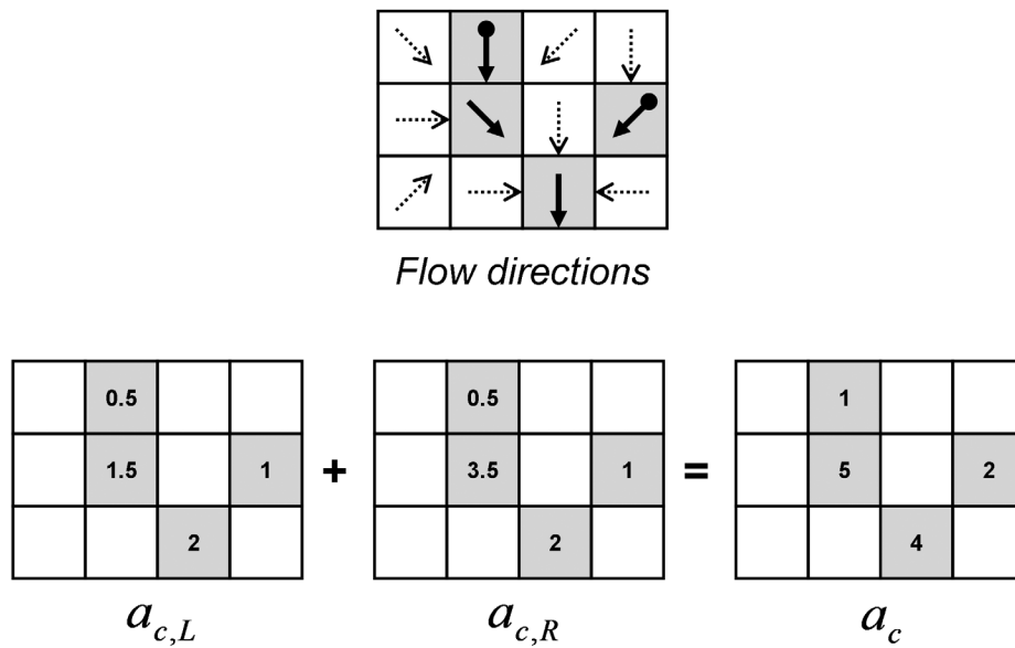
Figure 4. Illustrations of a flow direction map and three maps showing values of specific lateral contributing area, a_c . The flow direction map shows hillslope and stream flow directions. The three lower maps feature a_c entering the stream from left ( a_{c,L} ) and a_c entering the stream from right ( a_{c,R} ) as well as the total a_c , which is the sum of a_{c,L} and a_{c,R} . For simplicity, the a_c values presented in this illustration are equal to the number of contributing grid cells.
