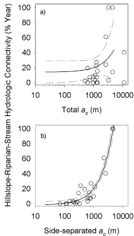
Figure 8. Hillslope a_c regressed against the percentage of the water-year that a hillslope-riparian-stream water table connection existed for 24 well transects. (a) Total a_c from both sides of a transect cross-section and (b) a_c separated into left and right sides of the stream. A connection occurred when there was stream flow and when water levels were recorded in both the riparian and hillslope wells (modified from Jencso et al. [2009]).
