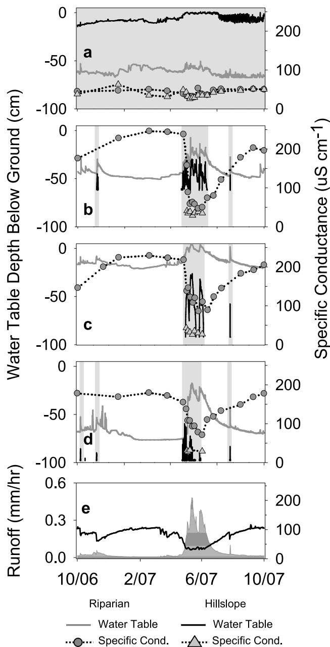
Figure 3. (a–d) Time series of riparian and hillslope water table dynamics and specific conductance at transects 1–4. Times of hillslope-riparian-stream hydrologic connectivity are indicated with gray shading. Runoff (dark gray shading) and specific conductance (black line) dynamics at the Lower Tenderfoot Creek flume are shown (e) for comparison to the transect dynamics.
