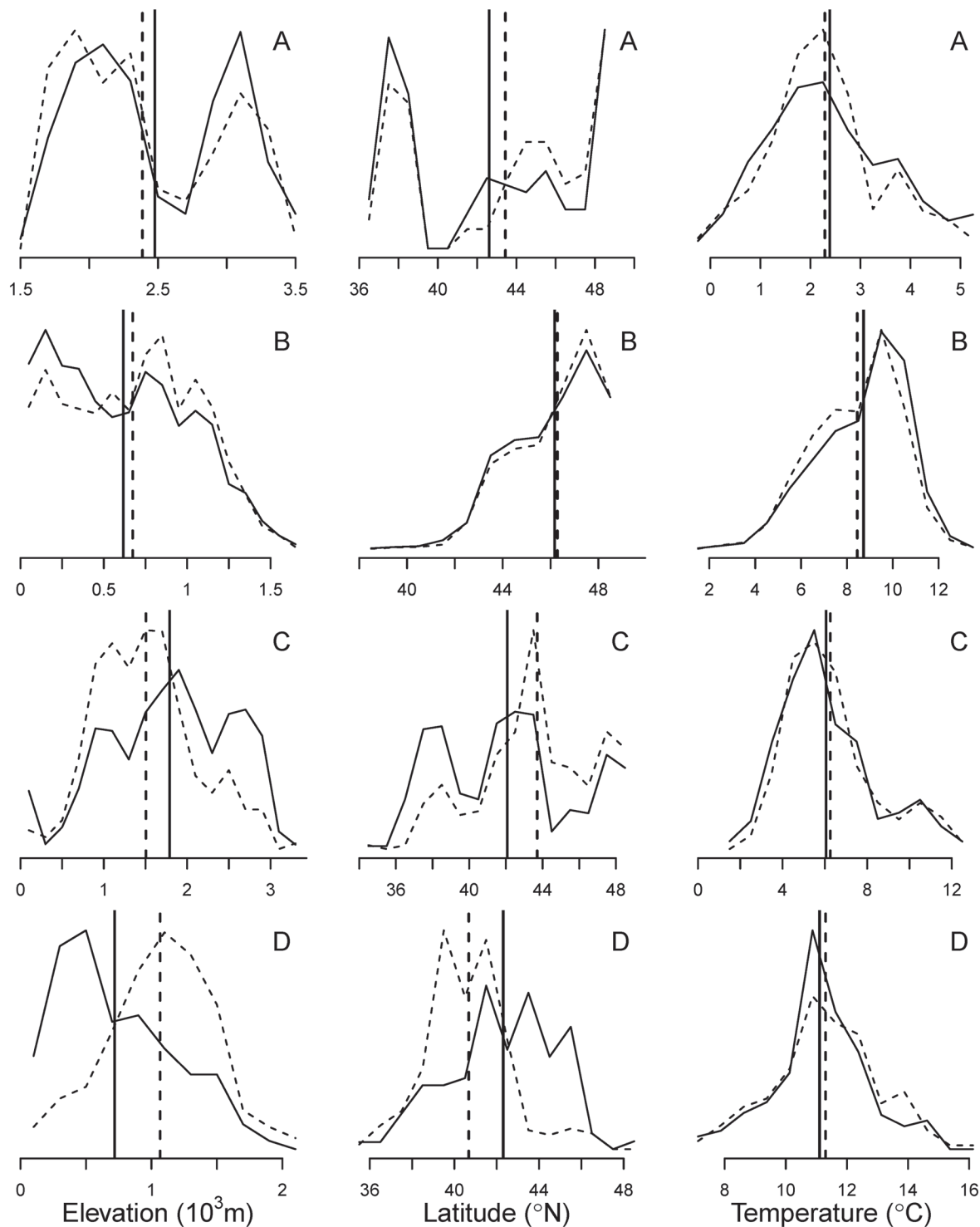
Fig 6. Estimated probability density functions of the elevation, latitude and temperature of the range of selected species. (A) Pinus albicaulis ; (B) Tsuga heterophylla ; (C) Pinus monticola ; (D) Cornus nuttallii . The solid line represents the distribution of mature trees and the dashed line the distribution of seedlings. Vertical lines represent the estimated mean of the distribution. The first column shows the elevation, the second latitude, and the third mean annual temperature. Ordinates are not shown because the figures are scaled so that the area under the curves is 1.
