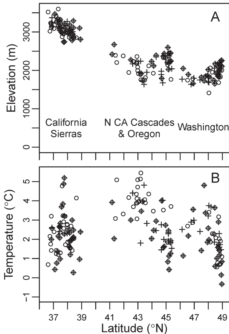
Fig 4. Distribution of plots with Pinus albicaulis . Open circles represent plots with trees, and crosses, plots with seedlings. (A) Elevation and (B) mean annual temperature, as a function of plot latitude.
