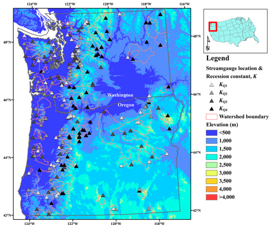
FIG. 1. Stream gauge locations (triangles) for 217 study watersheds with drainage boundaries (red lines) and shaded elevation map. Watersheds were divided into groups based on quartiles and shaded from light gray ( K_{Q1} ) to black ( K_{Q4} ): 0.810 \leq K_{Q1} < 0.941 , 0.941 \leq K_{Q2} < 0.950 , 0.950 \leq K_{Q3} < 0.963 , and 0.963 \leq K_{Q4} < 0.989 .
