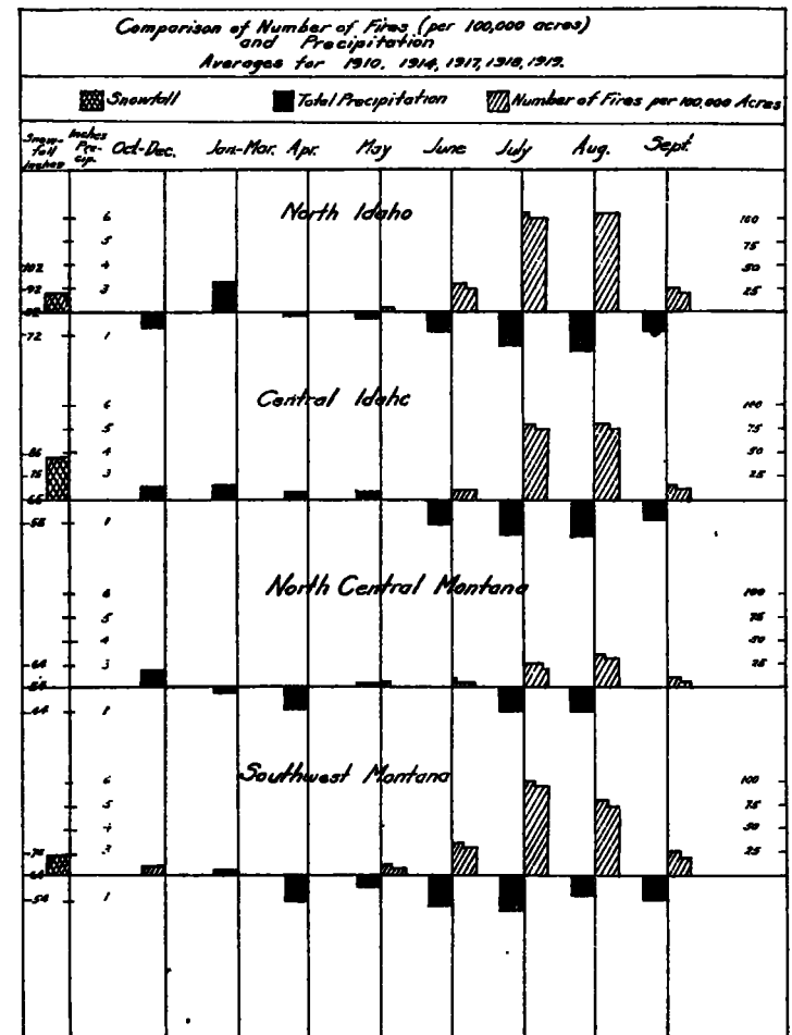
FIG. 9.—Relation of rainfall deficit to forest fires for the years 1910, 1914, 1917, 1918, and 1919, in north Idaho, central Idaho, north-central and southwest Montana.
