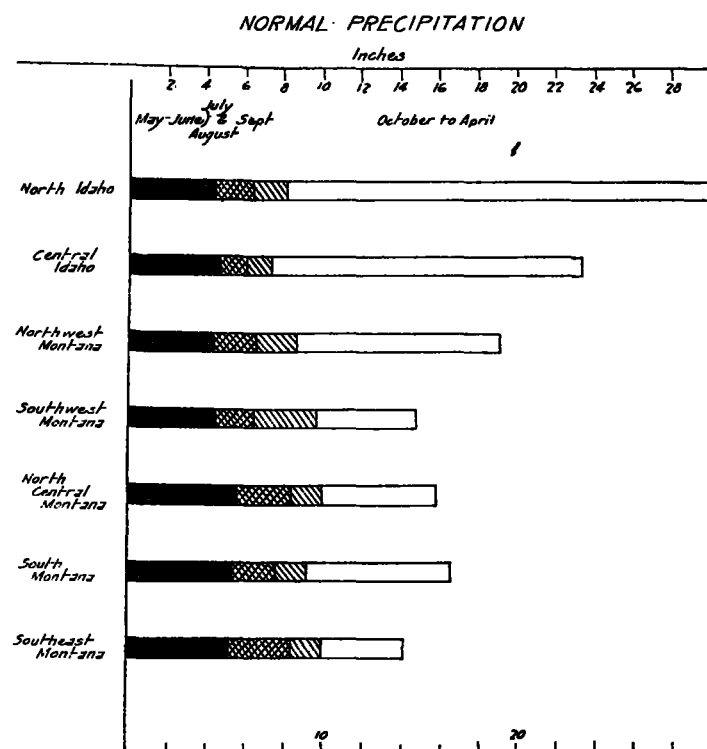
FIG. 5.—Precipitation by months for the seven climate sections of Montana and north Idaho.
