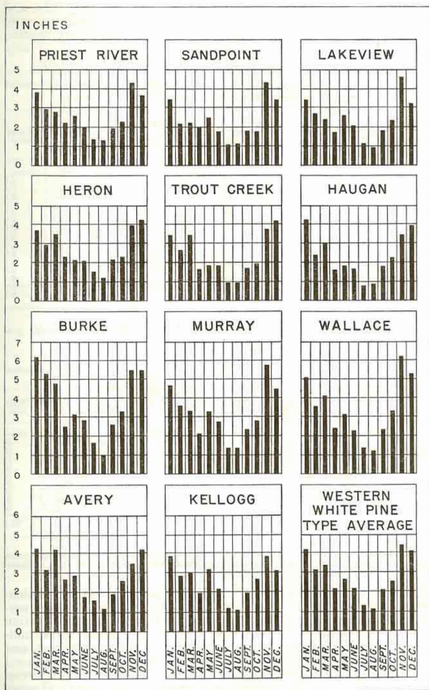
FIGURE 6.—Monthly distribution of precipitation in the western white pine region.
