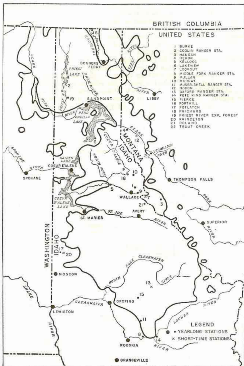
FIGURE 4.—Location of year-long and short-time weather stations in and near the western white pine region.
