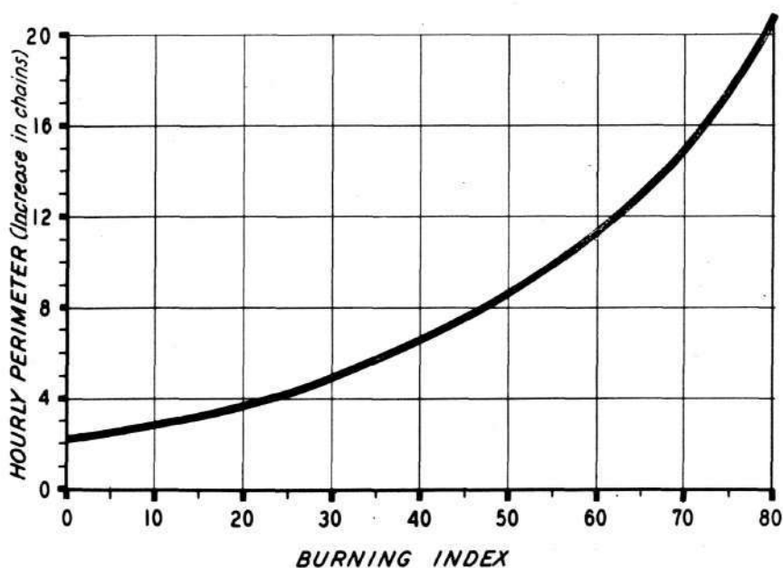
Figure 24. Average rate of spread from discovery to first attack according to burning index. (Basis 2953 fires, national forests, R-1, 1936-1948)
