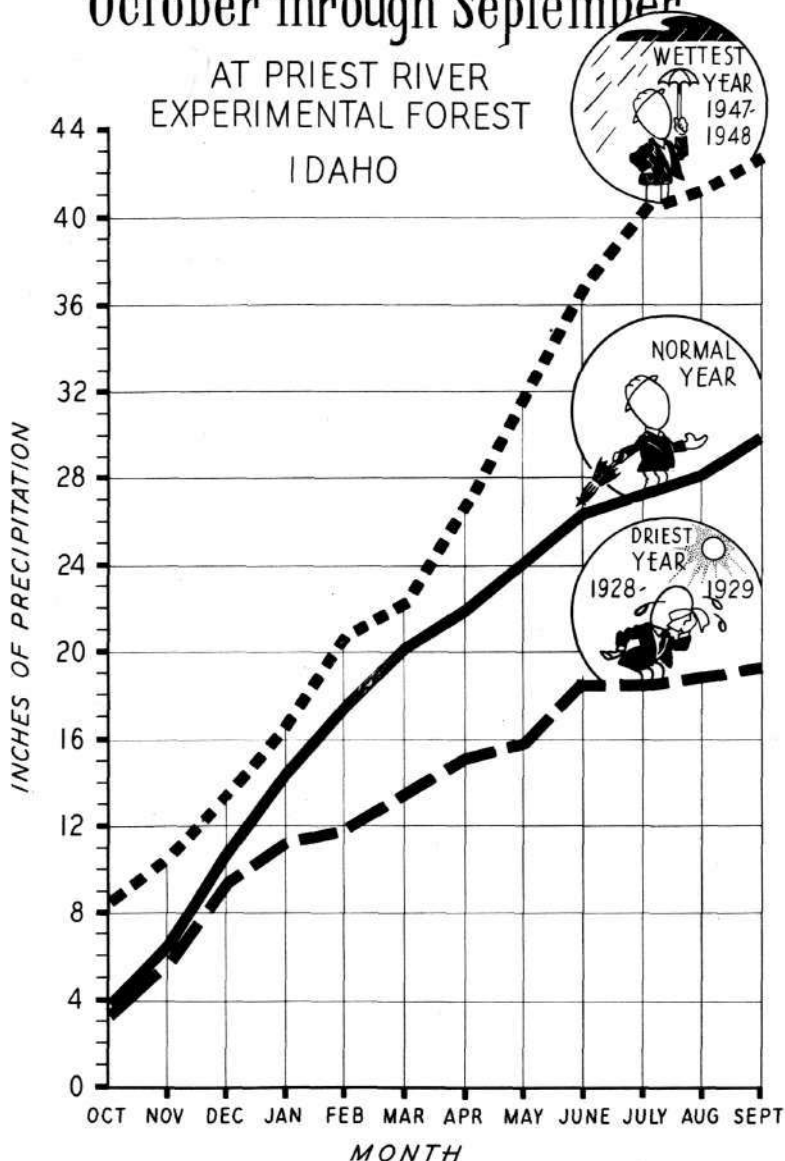
Figure 14. Cumulative precipitation, October through September, at Priest River Experimental Forest in wettest, normal, and driest years.
