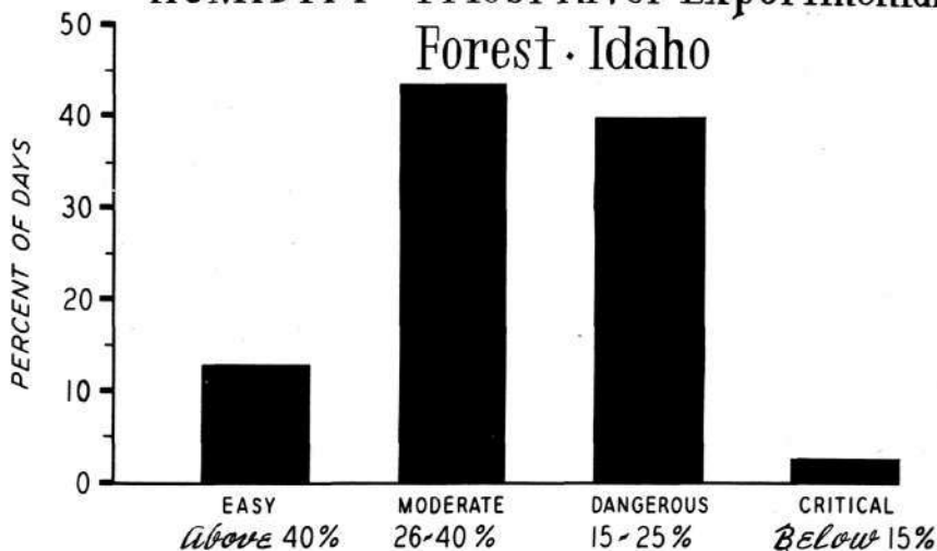
Figure 17. Frequency of occurrence of each relative humidity class during July and August at the Priest River Experimental Forest, Idaho.
