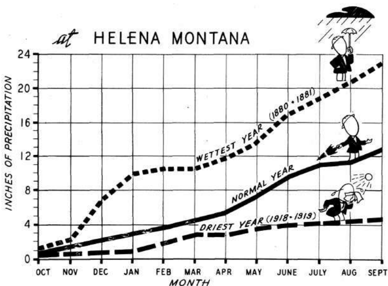
Figure 15. Cumulative precipitation, October through September, at Missoula, Montana, and Helena, Montana, in wettest, normal, and driest years.
