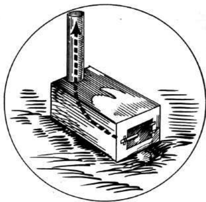
Figure 41. Box canyons and chimneys created by sharp ridges provide avenues for intense updrafts.
