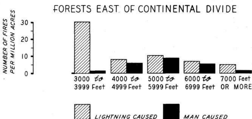
Figure 34. Average annual number of fires per million acres in each 1000-foot elevation zone in forests east and west of the Continental Divide. (Basis 16,793 fires, national forests, R-1, 1936-1944)
