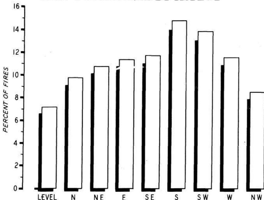
Figure 30. Percent of fires according to aspect at point of origin. (Basis 21,048 fires, national forests, R-1, 1931-1944)
