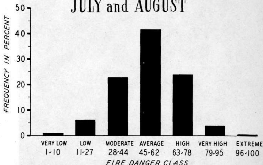
Figure 28. Frequency of occurrence of various classes of fire danger during July and August. (Basis 7440 daily observations on the 11 western national forests, R-1, 1936-1945)
