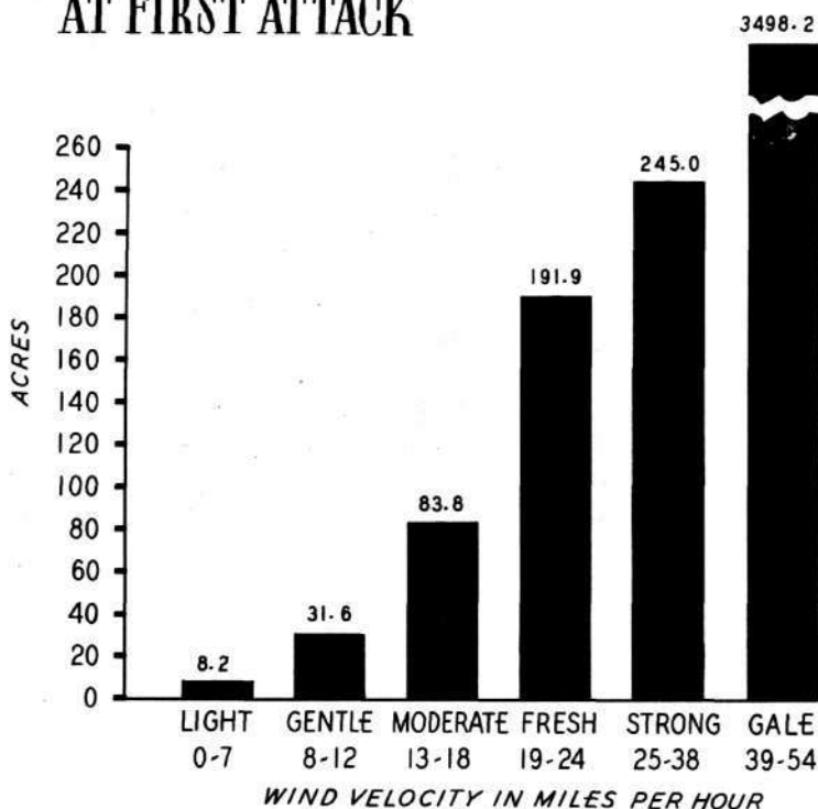
Figure 18. Average final size per fire in the national forests of Region 1 according to wind velocity at time of first attack. (Basis 12,790 fires, 1936-1944)
