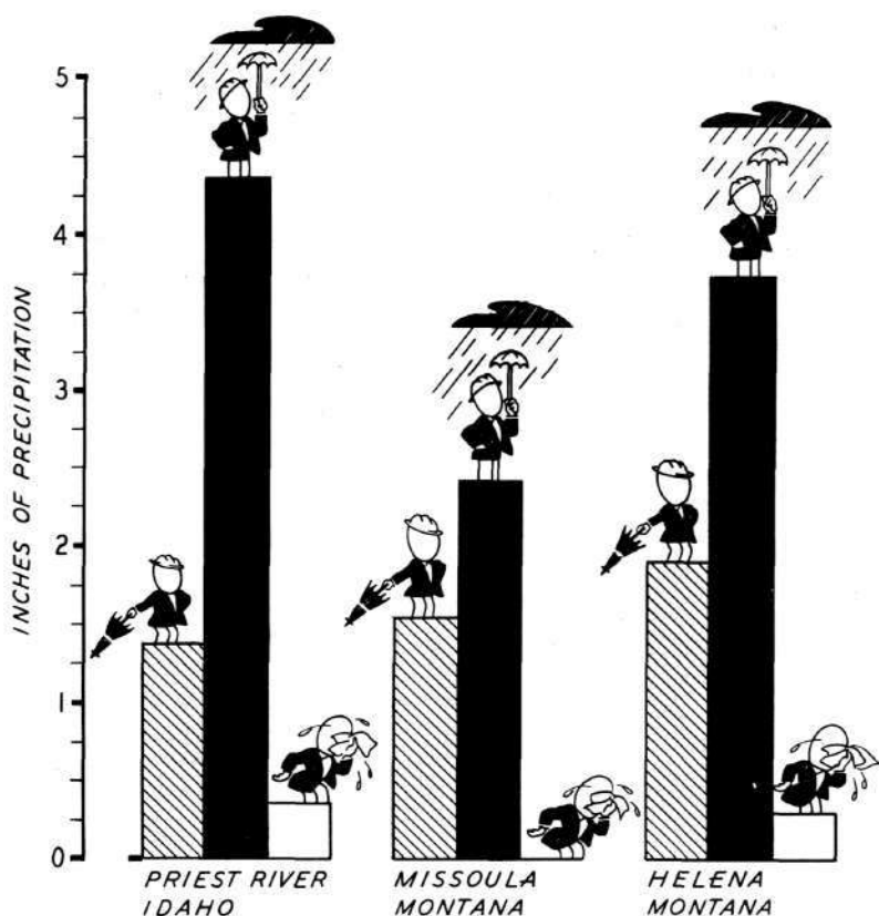
Figure 16. July and August precipitation at Priest River Experimental Forest, Idaho; Missoula, Montana; and Helena, Montana, during normal, wettest, and driest years.
