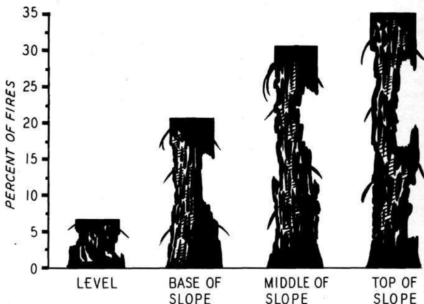
Figure 33. Percent of fires according to slope position at point of origin. (Basis 12,796 fires, national forests, R-1, 1931-1939)
