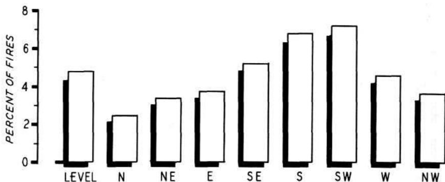
Figure 31. The percent of fires reaching large size increases steadily around the compass from north to south. (Basis 21,048 fires, national forests, R-1, 1931-1944)
