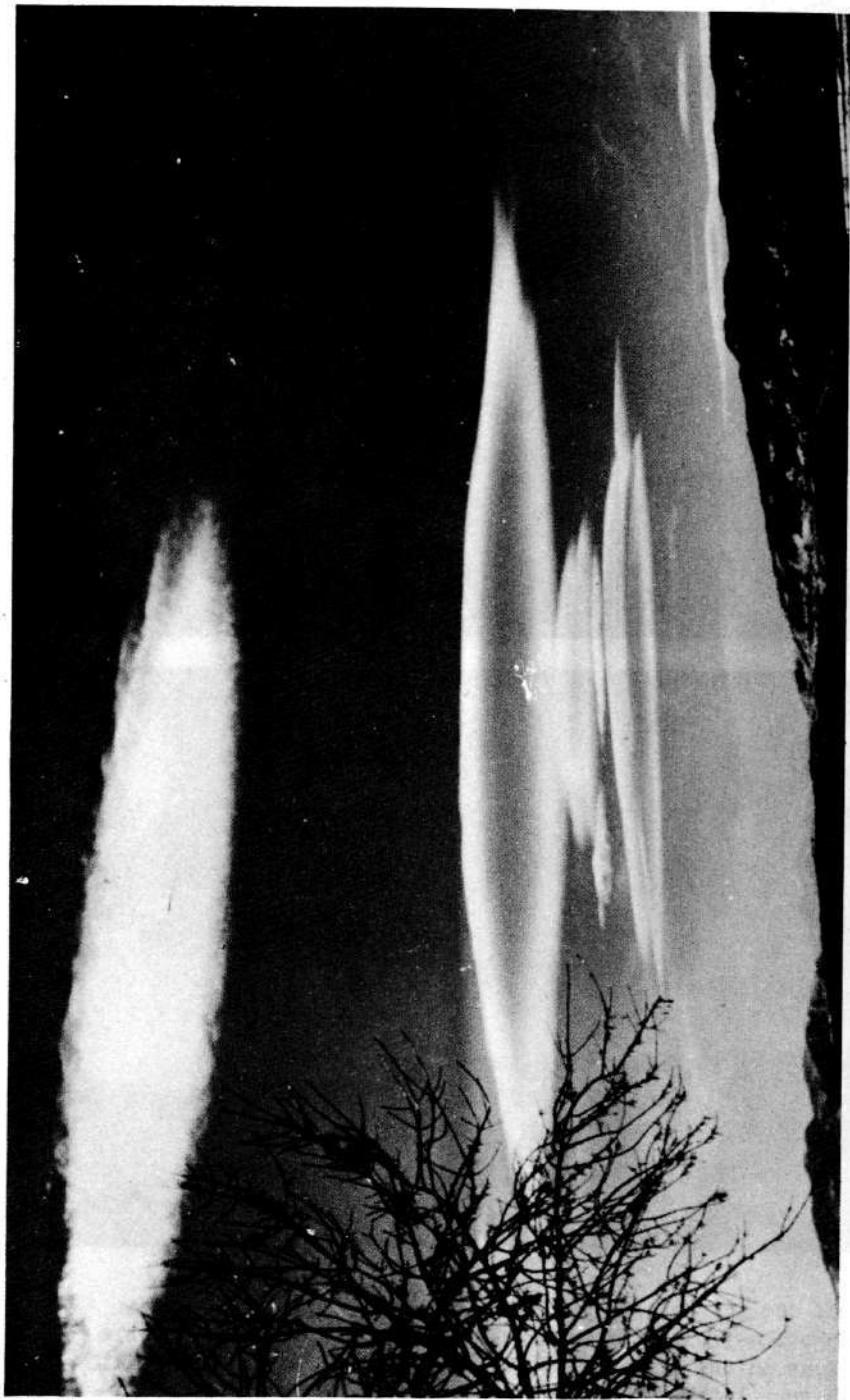
Figure 21. Lenticular clouds (altocumulus lenticularis) indicate high wind velocities at upper elevations and may be the warning signal that winds will increase at the site of a fire. (Photo by Maxwell Parshall, U. S. Weather Bureau)
