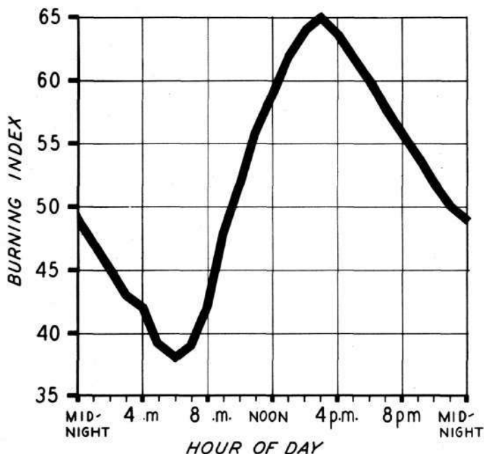
Figure 26. Average daily variation in burning index on a typical mid-summer day at the Priest River Experimental Forest. (Basis July-August observations, 1936-1939)
