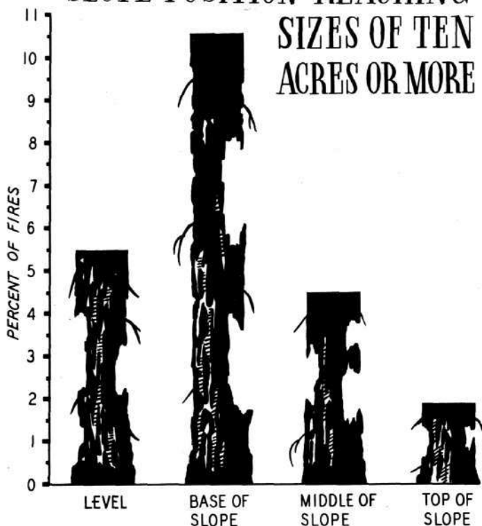
Figure 35. More fires starting at the base of the slope reach large size because a greater fuel area is available for spread of the fire. (Basis 12,796 fires, national forests, R-1, 1931-1939)
