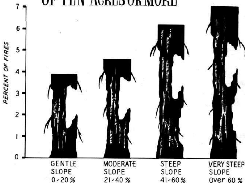
Figure 36. As slope steepness increases, a higher percentage of fires reach large size. (Basis 21,158 fires, national forests, R-1, 1931-1944)
