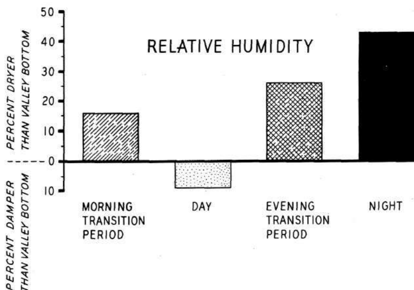
Figure 32. Variations in temperature and relative humidity during July and August between mountain tops and valley bottoms at Priest River Experimental Forest, Idaho. (Basis 1936-1939 measurements at weather stations located at 2300 feet and 5600 feet above sea level)
