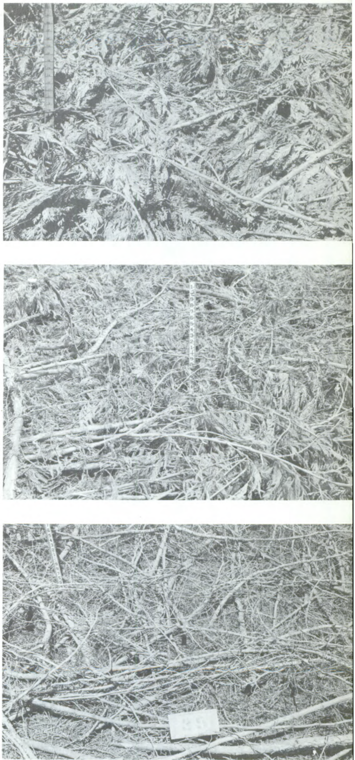
Figure 5. Slash of western redcedar, whose sprays disintegrate gradually in no set pattern (32.5 tons per acre). Upper , year of cutting; middle , 1 year after cutting; lower , 3 years after cutting.
