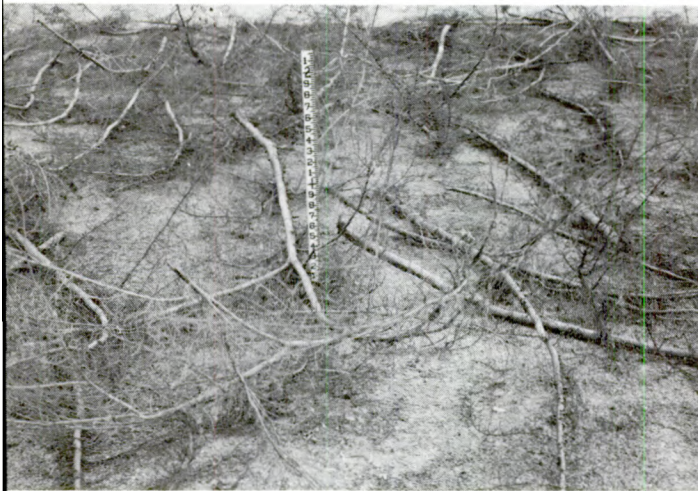
Figure 9. Variation in continuity within the fuel bed. Upper , continuous fine fuel in western white pine slash due to moderately fine branching and even distribution of needles; middle , discontinuity in western hemlock slash due primarily to loss of needles; lower , discontinuity in ponderosa pine slash due to coarse branching and tufted foliage (all species 7.5 tons per acre).
