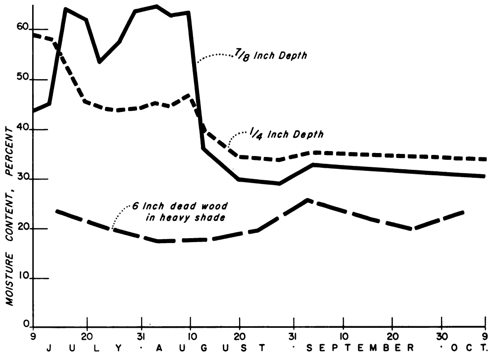
Figure 12. Drying rate of 6-inch wood of freshly cut tops, and comparison with older wood: upper , in full sun; lower , in shade.
