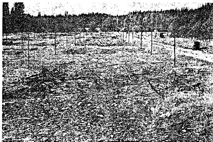
Figure 4. Five-year-old light slash (7.5 tons per acre) of: upper, western white pine; middle, western hemlock; lower, ponderosa pine. Aging has pretty well cancelled out original differences in fuel continuity. [Cf. (3) figure 9.]
