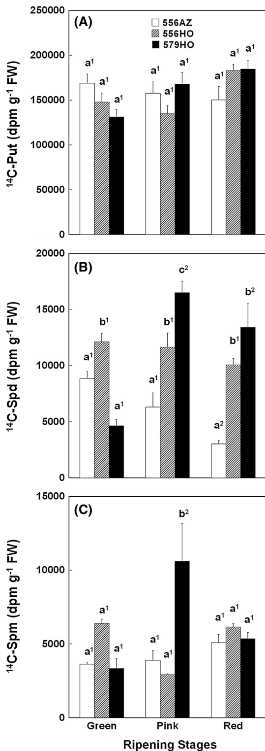
◀ Fig. 5 The amount of radioactivity from L-[U- ^{14}\text{C} ]-putrescine present as free putrescine (A), spermidine (B), and spermine (C) in tomato fruit pericarp (at different stages of ripening) of 556AZ, 556HO and 579HO lines. The incubation time was 8 h. Data are mean \pm SE of four replicates. Statistically significant differences ( P \leq 0.05 ) among the genotypes at a given stage of ripening are indicated by different letters , and the differences within the same genotype at different stages of ripening are indicated by different numbers
