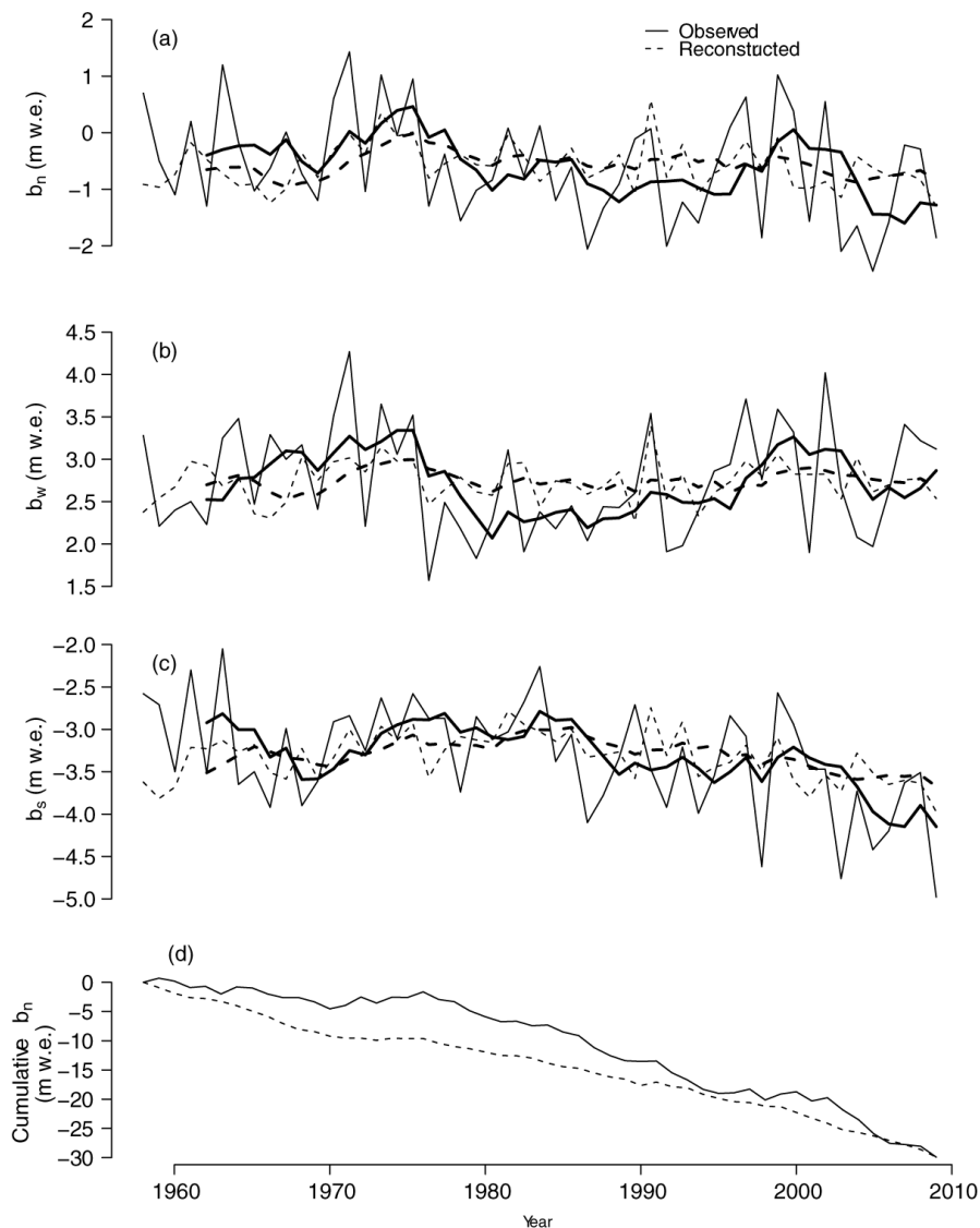
Figure 2. Fitted net ( b_n ), winter ( b_w ), and summer ( b_s ) mass balance (dashed line; meters water equivalent [m w.e.]) plotted against the corresponding observed balance values (solid line) for the measurement period of 1959–2009. Net balance (a) is fitted from residuals PC1, winter balance (b) is from the Minotaur Lake residual chronology, and summer balance (c) used the Hidden Lake residual chronology. A 5-year running mean has been fit to the reconstructed balance (thick dashed line) and the observed balance (thick solid line) to highlight patterns in the shorter measurement period. The bottom graph (d) is a comparison of reconstructed and observed cumulative net mass balance over the measurement period.
