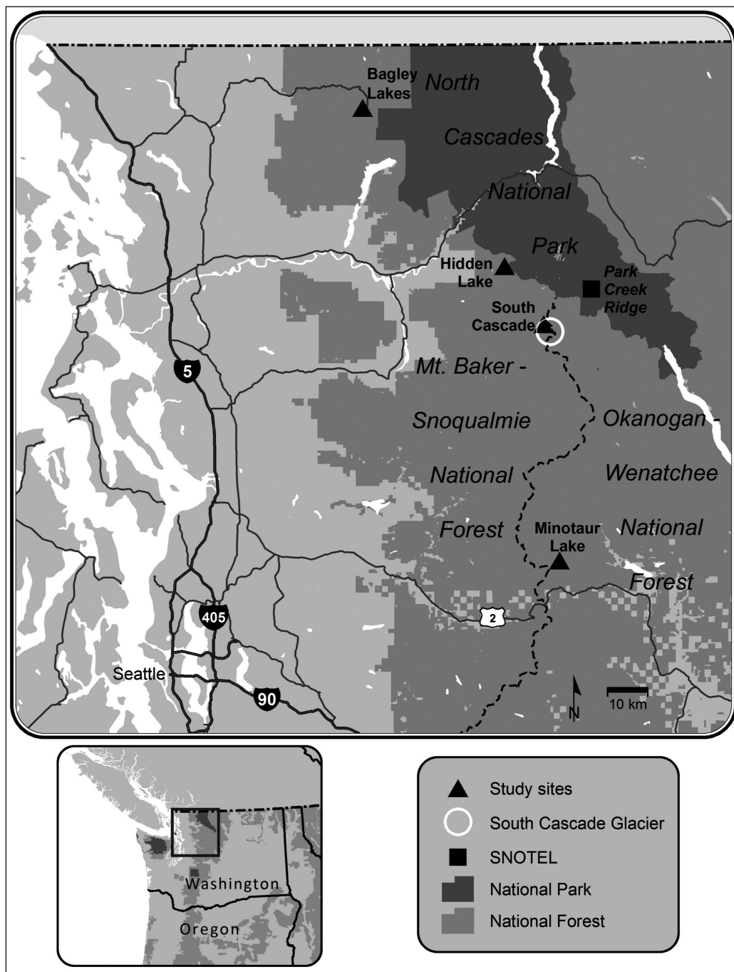
Figure 1. Map of study sites. Triangles represent sampling locations, the white circle represents the location of South Cascade Glacier, and the square represents the SNOTEL site used in the climate-growth correlations. Shaded light gray areas indicate National Forest lands, and shaded dark gray areas indicate National Parks.
