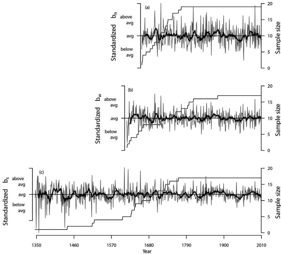
Figure 3. Time series plots of reconstructed net ( b_n ), winter ( b_w ), and summer ( b_s ) mass balance. Net balance (a) is reconstructed from PC1 for 1659–2009, winter balance (b) is reconstructed from the Minotaur Lake residual chronology for the span 1615–2009, and summer balance (c) is reconstructed from the Hidden Lake residual chronology, 1346–2009. The thick black line represents a 10-year moving average. Sample depth is indicated by the thin black line and the right side y-axis, where sample depth for (a) indicates the shortest chronology entered into the PCA. These plots have been standardized by adding in the mean for each individual series in order to show a clearer picture of periods of above- and below-average balance.
