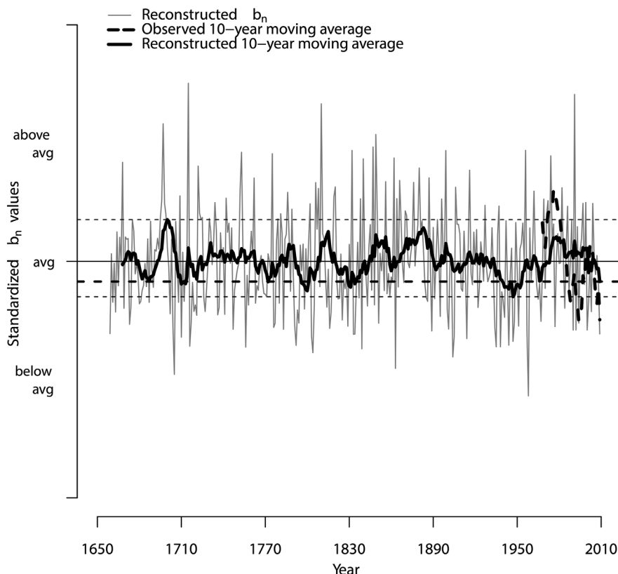
Figure 7. Time series plot of reconstructed and observed net balance ( b_n ). The thick solid line represents a 10-year moving average of the reconstructed balance, and the thick dashed line is a 10-year moving average for the observed net balance. The thin dashed lines represent the minimum and maximum values of the reconstructed moving average line. The thick long dashed line represents the reconstructed moving average minimum for 2009. All series have been standardized by adding in the mean for each individual series in order to show a clearer picture of periods of above- and below-average balance.
