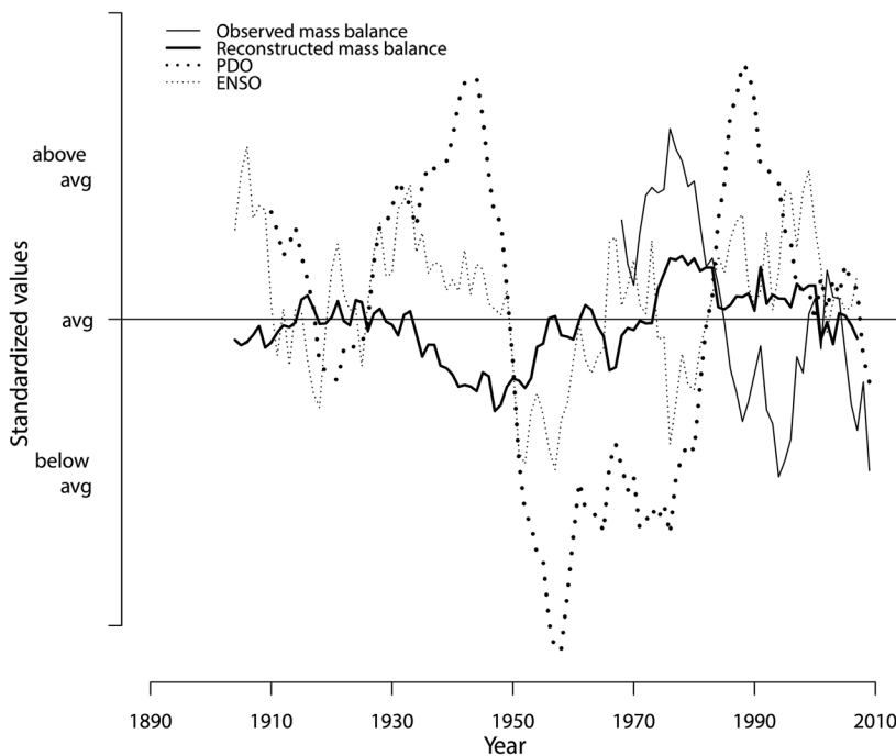
Figure 5. Time series plot of reconstructed net mass balance, observed net mass balance, average winter Pacific Decadal Oscillation (PDO) index values, and average winter Niño 3.4 (ENSO) index. The series are displayed as a 10-year moving average and have all been standardized
