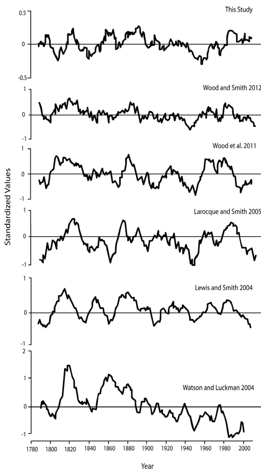
Figure 4. Comparison of the reconstructed net balance created in this study to reconstructed net balance created in similar studies in the Pacific Northwest. Adapted from Wood et al. (2011) and Wood and Smith (2012). The scales and magnitudes of the reconstructions are different and some caution should be taken when interpreting standardized values on the y-axis. The last decade of the South Cascade Glacier reconstruction created in this study is not shown.
