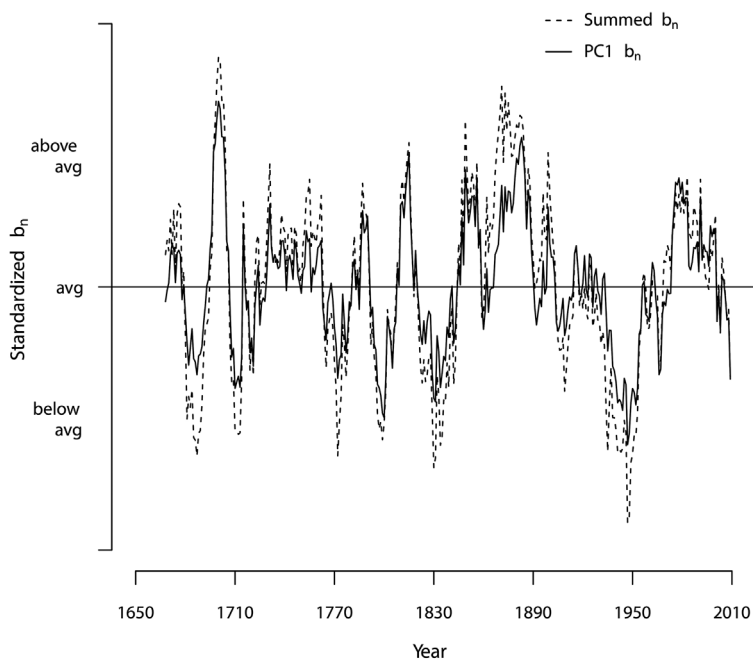
Figure 6. Time series plots of reconstructed net balance. The solid line represents a 10-year moving average of net balance reconstructed from PC1, and the dashed line represents a 10-year moving average of net balance from the sum of the winter and summer mass balances. These series have been standardized.
