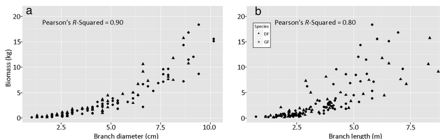
Figure 1 Scatterplot of dry biomass (kg) against branch diameter (a) and branch length (b) by species (DF = Douglas-fir, GF = Grand fir).
