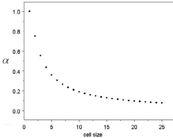
Figure 3 Effective location error \alpha as a function of cell size. Cell size is shown here in multiplies of pixels, where average location error is set to 1 pixel in both x and y directions. Cell size varies between 1 and 25 times the magnitude of location error.
