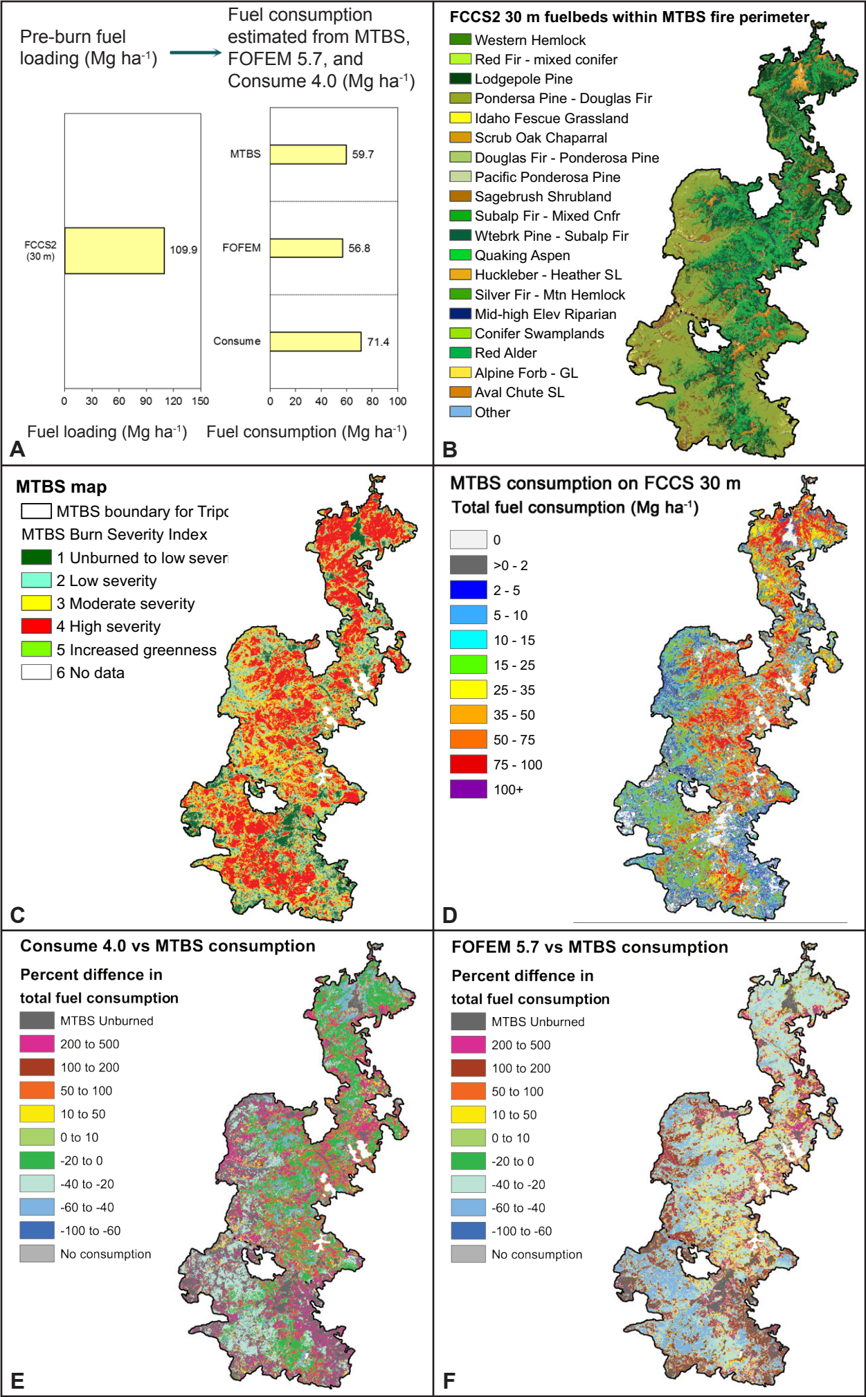
Figure 8. Fuel consumption estimated from MTBS linked to Composite Burn Index (CBI) and compared with Consume 4.0 and FOFEM 5.7 fuel consumption outputs. All results shown are based on the MTBS fire perimeter and FCCS2 30 m fuelbeds for the Tripod Fire Complex. This figure shows (A) the fuel loading and fuel consumption estimates from MTBS, FOFEM, and Consume; (B) the FCCS2 30 m vegetation map; (C) burn severity; and (D) the corresponding fuel consumption calculated from burn severity and CBI. Also shown in panels (E) and (F) are the differences (%) in fuel consumptions between MTBS and Consume (E) and MTBS and FOFEM (F).
