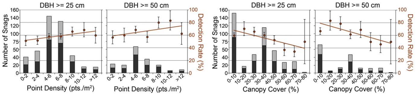
Fig. 10. Lidar point density and canopy cover detection rate trends for two different \geq DBH class scenarios (DBH \geq 25 cm and 50 cm). Black and gray bars represent the proportion of detected and undetected snags respectively for the individual point density and canopy cover classes.
