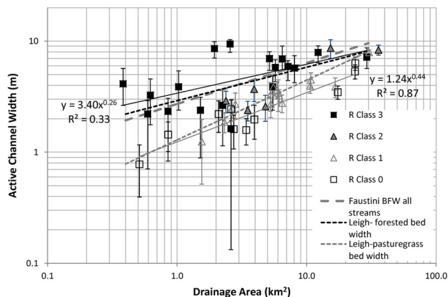
Figure 2. Relationship of active channel width versus drainage area for different observed reach-scale riparian conditions. Each point is the mean of 31 active channel widths taken over each 150-m reach, and whiskers portray plus and minus one standard deviation of the active channel widths in each reach. Power functions are fitted to the riparian class 0 and class 3 streams. Leigh's (2010) bed width relationships for two drainages in the Upper Little Tennessee closely match the active channel width relationships collected here. The regional bankfull width (BFW) relationship of Faustini et al. (2009) for both disturbed and undisturbed Southern Appalachian streams is shown in the dashed grey line.
