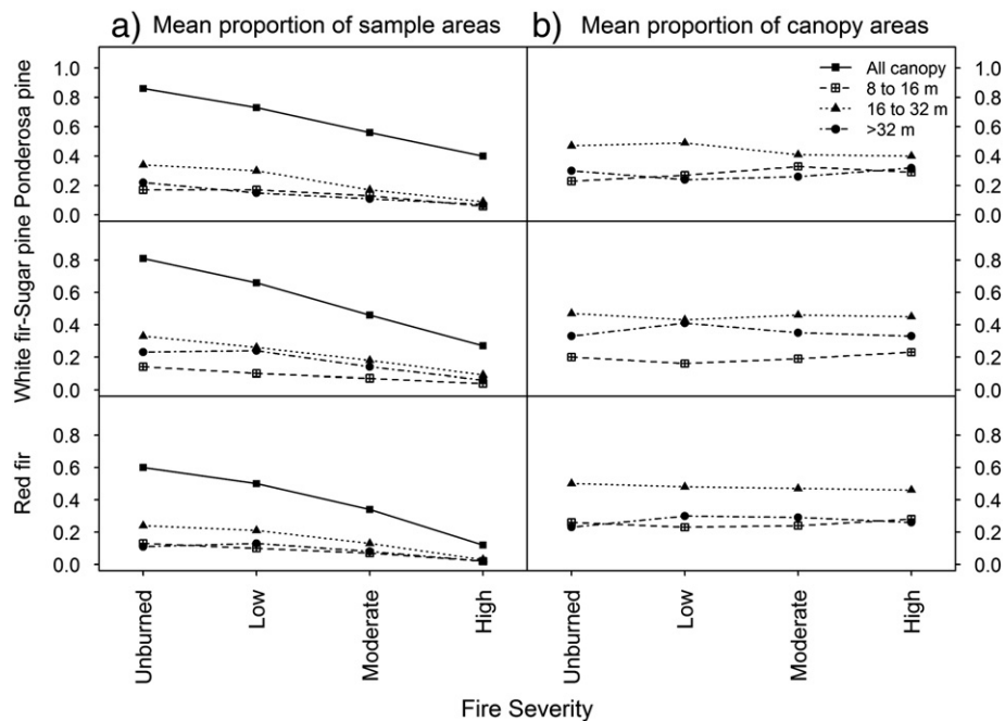
Fig. 7. Change in proportion of canopy area by forest type and fire severity. As fire severity increases, the absolute area of canopy cover decreased in all strata (a). However, within the remaining canopy area, the proportion of area in different strata showed little change (b), indicating that fire left multistory tree clumps. Because the absolute area of 2–8 m canopy increased for two forest types with increasing fire severity, the method for calculating proportion of canopy area (b) was calculated using canopy area minus the 2–8 m canopy area. See Fig. 8 for changes in the 2 to 8 m canopy stratum.
