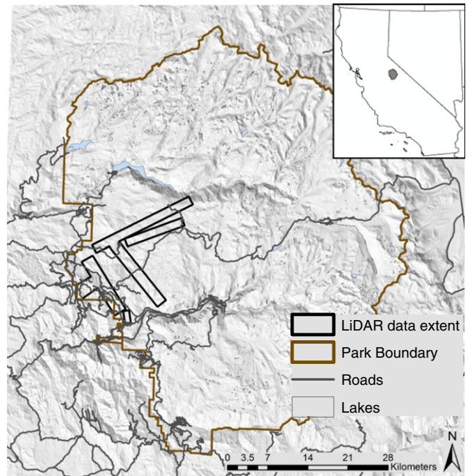
Fig. 2. Location of LiDAR data collection (bold black lines) within Yosemite National Park. Inset shows location of park within the state of California. Supplement Fig. S1 and Fig. S2 show higher resolution maps of the study area.
