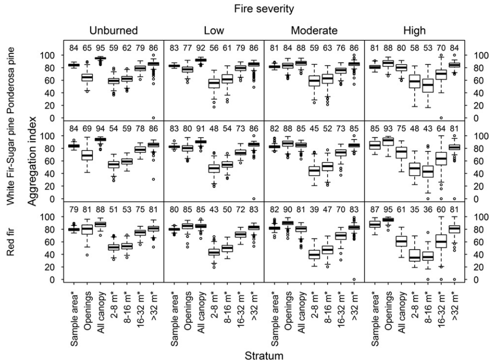
Fig. 10. Clumping of openings and canopy strata (class types) within larger patches as opposed to dispersion based on the Fragstats aggregation index. Aggregation value (numerical value above each bar and whisker plot) was calculated as the likelihood that an adjacent cell is of the same patch type. Higher values indicate greater clumping into fewer, larger patches. As fire severity increased, openings became more aggregated while overall canopy patches became smaller and more dispersed. Aggregation of patches within individual canopy strata, however, showed only modest changes. Results calculated for each sample area are based on a classification of only openings (<2 m) and all canopy (>2 m) and by height strata (indicated with an asterisk in legend). Bold lines show median values; the bottom and top of the boxes show the 25th and 75th percentile values; the upper and lower whiskers show either minimum and maximum values or 1.5 times the interquartile range (approximately two standard deviations), whichever is nearer to the mean; and circles show outliers. See Supplement Fig. S5 for aggregation values calculated relative to a random distribution of cells by height strata.
