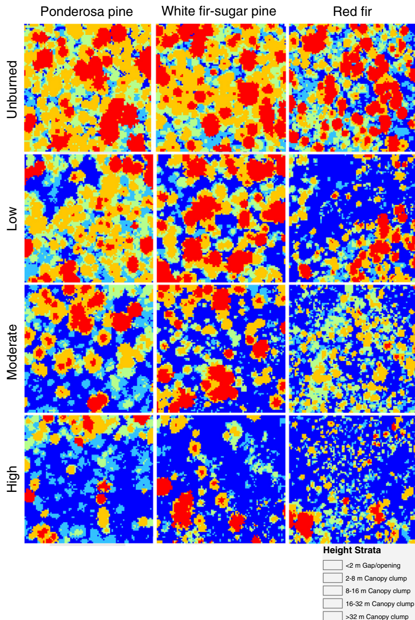
Fig. 4. Example sample areas (0.81 ha) for each forest type-fire severity combination. Examples illustrate common spatial patterns but not the range of variation found for each combination.
