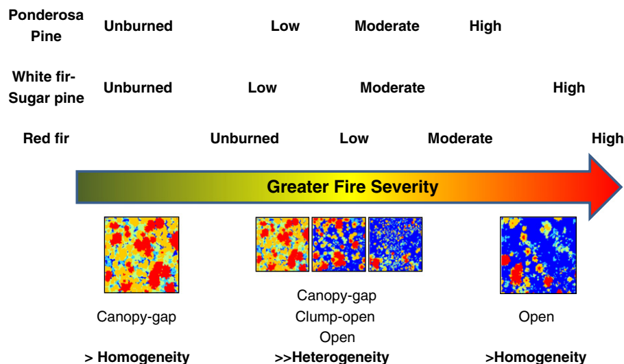
Fig. 11. Changes in spatial structure comparing unburned (outside all fire perimeters since 1930) and burned areas with increasing fire severity. While the direction of change with fire severity was consistent across forest types, each forest type was unique in the range of structures found along this general continuum. Forest types are shown above the line. Fire severities shown for each forest type line up with the characteristic canopy and opening structures shown below the arrow for that forest type and fire severity.
