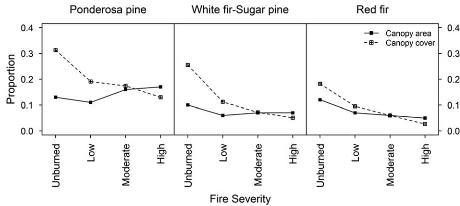
Fig. 8. Change in proportion of canopy area and canopy cover by forest type and fire severity in the 2 to 8 m stratum. Canopy cover trends suggest ‘thinning from below’ in this stratum as fire removes smaller trees under larger trees and standalone tree clumps in this stratum. Increases in canopy area with increased fire severity suggests establishment of new tree clumps in this stratum through regeneration. Canopy cover uses the total vertical distribution of returns as an estimate of the canopy profile and estimates the presence of canopy at all heights whether or not there is foliage above a given height. Canopy area measures only the top of canopy foliage in each 1 m grid cell and ignores lower foliage and therefore measures the area of top-of-canopy trees within clumps.
