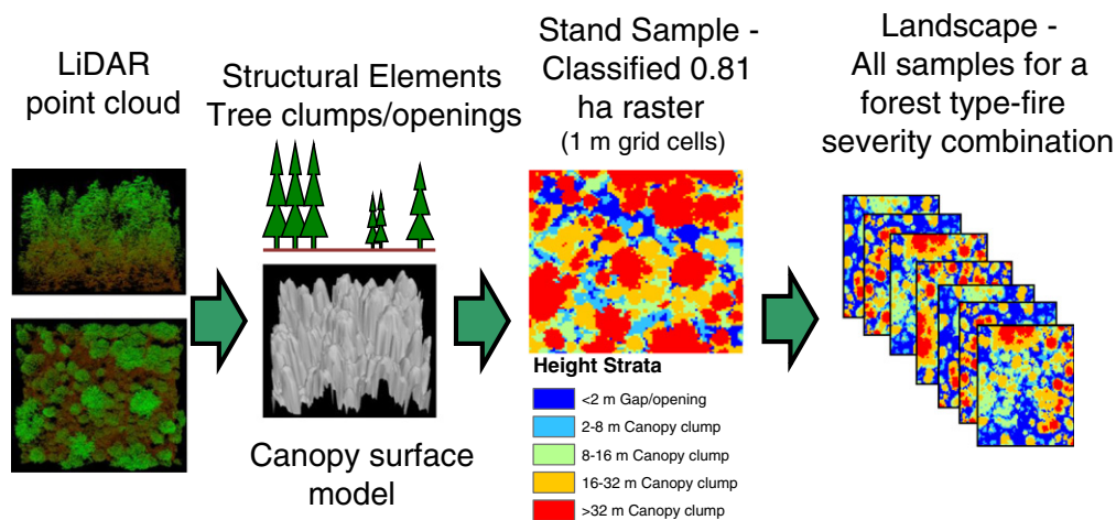
Fig. 3. Methods used to identify gaps/openings and canopy patches in different strata—and to analyze spatial structure. Individual tree clumps and openings were identified from 90 \times 90 m canopy surface models produced from the LiDAR point cloud (sample areas). Each 1 m CSM grid cell was classified into a height stratum to identify canopy clumps and openings. Analysis was done on patterns of structural elements within each sample area to understand structure within stands. Analysis of all sample areas for a given forest type and fire severity combination was done to reveal landscape patterns.
