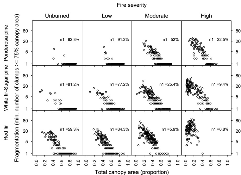
Fig. 9. Fragmentation of canopy clumps within sample areas. As fire severity increased, the total area in canopy (x axis) decreased while the number of clumps (y axis) increased indicating progressive fragmentation of remaining canopy into smaller clumps. Each point represents one sample area. To exclude small clumps that made little contribution to total canopy area, clump count was calculated by determining the minimum number of clumps within each sample area required to account for 75% of canopy area with clumps added in order of size (largest first). The percentage of sample areas where all canopy in a single continuous clump (‘N1 =’), usually percolated with enclosed gaps, is shown.
