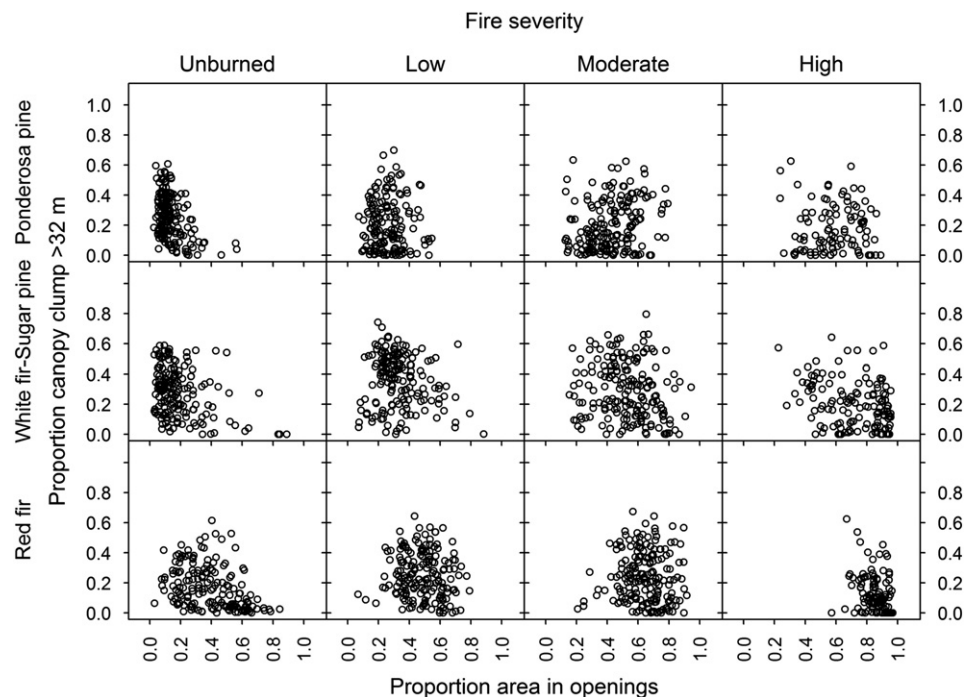
Fig. 5. Heterogeneity in total opening area and tall-tree (>32 m) patch areas by fire severity and forest type with the proportion of the total area in openings (x axis) and the proportion of total canopy area in tall tree (>32 m) clumps (y axis). Wider point dispersal indicates a greater range of structural heterogeneity for a given fire severity-forest type combination. Increased fire severity resulted in a greater range of opening area for ponderosa pine and white fir-sugar pine forests but resulted in a narrow range for red fir. Increased fire severity had little effect on the range of sample area proportions in tall tree clumps for either ponderosa pine or white fir-sugar pine forests but resulted in a narrower range for red fir. Supplemental Fig. S3 shows change in heterogeneity for other canopy strata.
