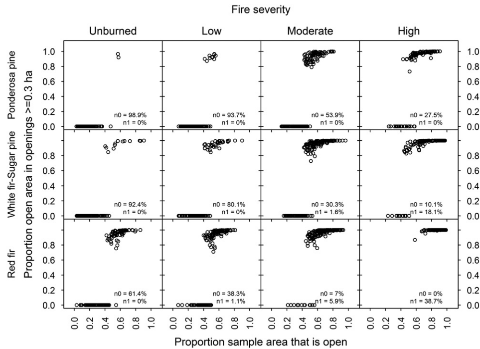
Fig. 6. Proportion of openings that are \geq 0.3 ha (needed for regeneration of tree species requiring high sunlight exposure) plotted against proportion of the total sample area in openings by fire severity and forest type. The percentage of sample areas where there are no gaps \geq 0.3 ('N 0 ='), and the percentage of sample areas where all openings are \geq 0.3 ha ('N 1 =') are shown.
