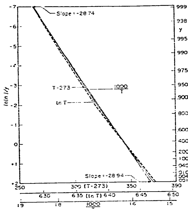
Fig. 1. Deviations from the linearity predictions of eqns (6), (7) and (8) for a heating rate of 5°C/min and a simple first-order reaction with A = 1.15 \times 10^{19} \text{ min}^{-1} and E = 55 \text{ kcal/mole} (from ref. 3).
