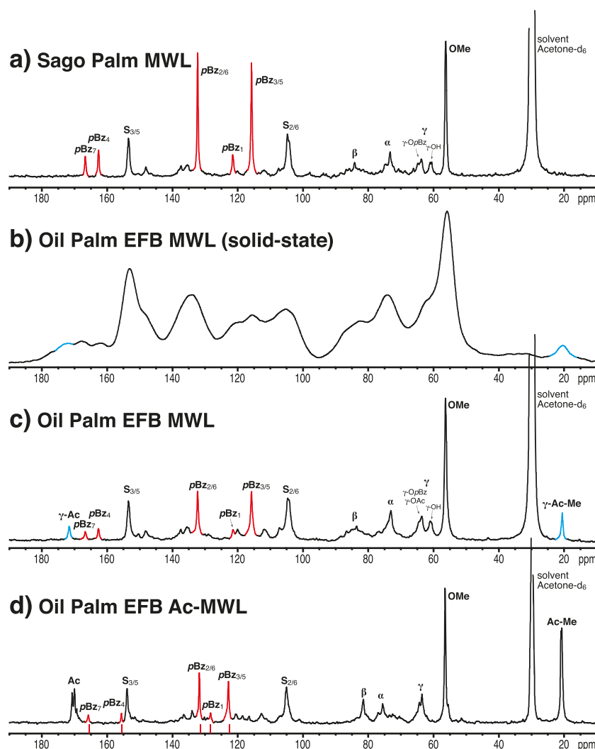
Fig. 1 1D ^{13}\text{C} NMR spectra of various palm lignins. a Solution-state spectrum from a sago palm MWL isolated as described previously [35]. b Solid-state (200 MHz) spectrum and c solution-state spectrum of MWL isolated from the oil palm empty fruit bunches (EFB) previously characterized [34, 43]. d Solution-state spectrum of acetylated EFB isolated lignin (Ac-MWL). The solution-state spectra were run at 400 MHz (100 MHz ^{13}\text{C} ); the acetylated MWL is in acetone- \text{d}_6 , underivatized MWLs in 9:1 acetone- \text{d}_6 : \text{D}_2\text{O} . Red-colored peaks labeled pBz are for carbons in the p -hydroxybenzoyl moiety. The red lines between plot d
