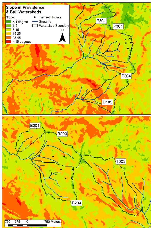
Figure 7. Slopes in the eight catchments are moderately steep as shown by a weighted scale ( < 1^\circ dark green; 1\text{--}5^\circ medium green; 5\text{--}15^\circ chartreuse; 15\text{--}25^\circ light orange; 25\text{--}45^\circ dark orange; > 45^\circ red). Flat areas in crest and depositional locations are very small. Slope values calculated from a 10 m digital elevation model. Mean annual sediment export is given for water years 2005–2011.
