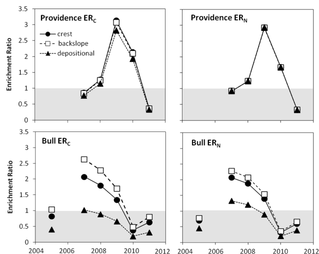
Figure 6. Enrichment ratios for carbon ( ER_C ) and nitrogen ( ER_N ) in material (<2 mm) collected from sediment basins at the outlet of each catchment over the water years 2005–2011. Different symbols represent enrichment ratios calculated using average surface mineral soil (0–10 cm) values for the three hillslope positions studied in Providence (low elevation) and Bull (high-elevation) catchments. Sediment basins were installed over the years 2002–2004 and archived samples were not preserved for many sediment basins in 2006 or before 2005.
