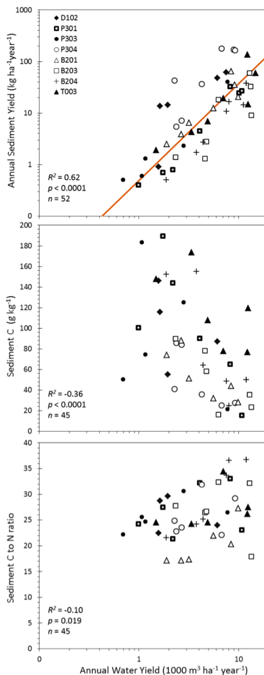
Figure 4. Top: annual sediment yield is directly correlated with annual water yield. Middle: annual sediment carbon (C) and nitrogen (N; not shown) concentrations have an inverse relationship to water yield. Bottom: the C-to-N mass ratio is weakly correlated with water yield. Data presented for WY 2005, and 2007–2011 (sediment basins constructed over the period 2002–2004, samples were not preserved for testing from WY 2006).
