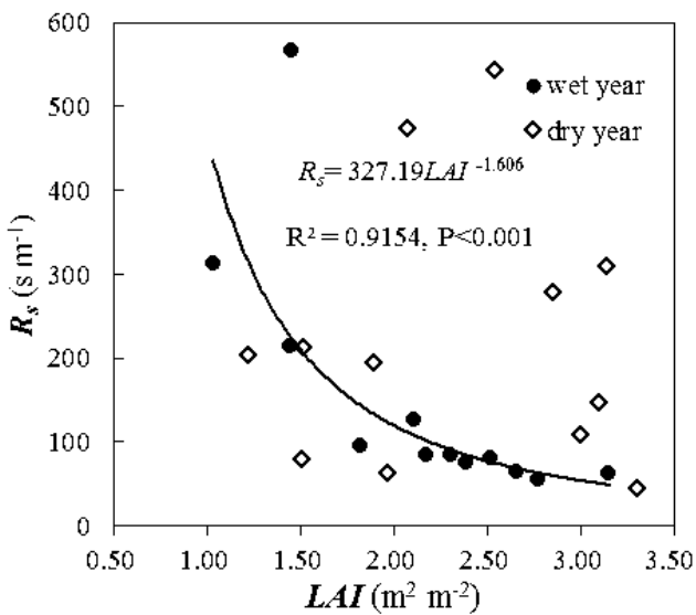
Figure 6. The relationship between leaf area index (LAI) and surface resistance ( R_s ) during the growing season of the wet and dry years.
