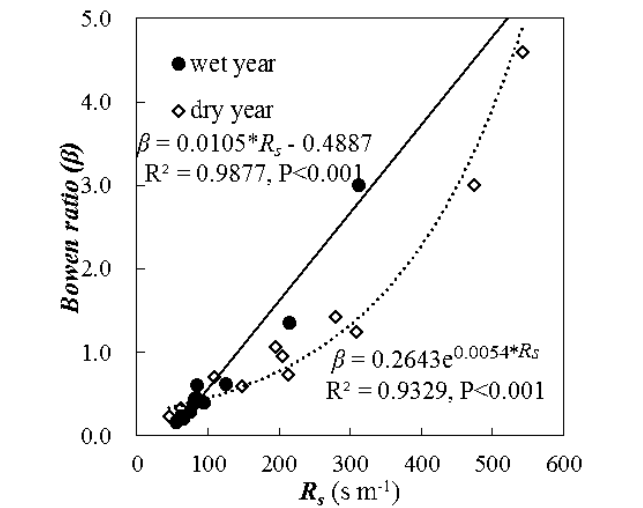
Figure 10. Response of monthly average Bowen ratio ( \beta ) on surface resistance ( R_s ) in the wet and dry years.
