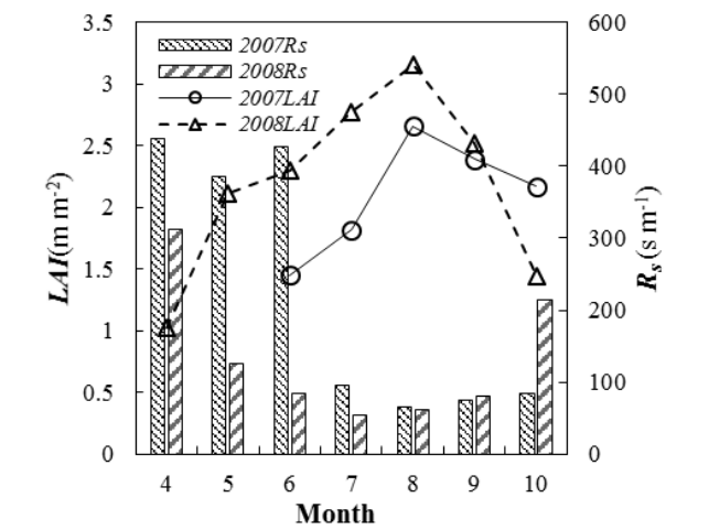
Figure 9. Seasonal variations of monthly average LAI and R_s during the growing seasons in the wet years of 2007 and 2008.
