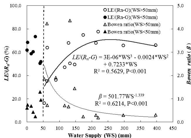
Figure 8. The response of Bowen ratio and LE/(R_n - G) to water supply (WS; including precipitation ( P ) and irrigation ( I ) during each individual period) of the different periods across the four growing seasons.
