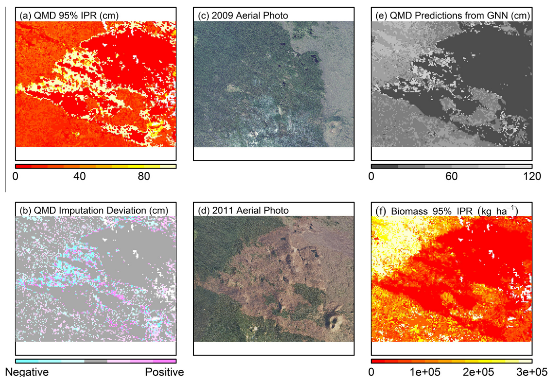
Fig. 5. Representation of the impacts of the Scott Mountain Fire west of Sisters, OR, on QMD predictions. We present spatial patterns in (a–b) QMD 95% IPR and imputation deviations in predictions from the bootstrap sample, (c–d) evidence of wildfire in the area, as shown by aerial photos taken in 2009 and 2011, and spatial patterns in (e) QMD predictions from GNN and (f) 95% IPR of biomass.
