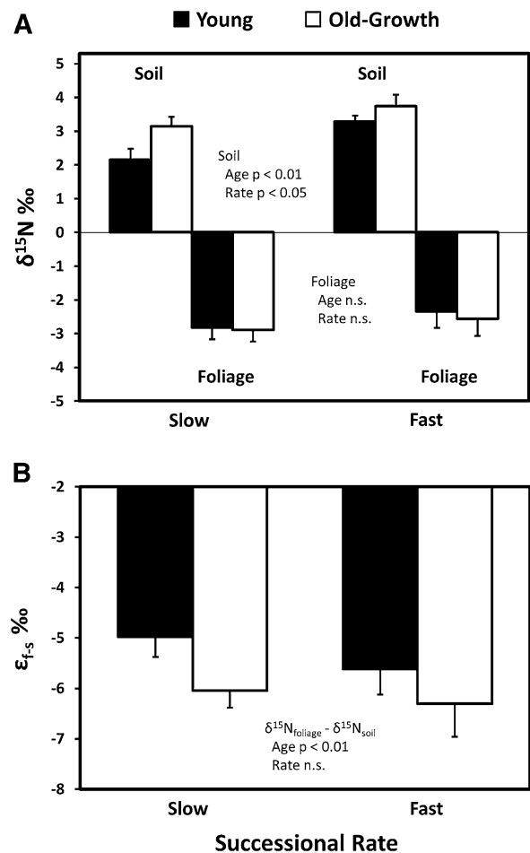
Figure 2. Successional rate and stand-age effects on (A) \delta^{15}\text{N} values in mineral soil (0–10 cm) and foliage and (B) \delta^{15}\text{N} span between foliage and mineral soil ( \epsilon_{f-s} ). Young stands are recovering from logging and broadcast burning, whereas old-growth stands are undisturbed. Error bars represent \pm 1 SE. Significant effects are shown in figure panels.
