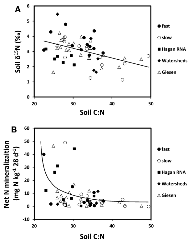
Figure 4. Mineral soil (0–10 cm) C:N versus (A) soil \delta^{15}\text{N} values and (B) N mineralization. Regression lines include all points; symbols distinguish groups of study sites for the 60 plots (see Table 1). Linear regression line for (A) y = -0.0649x + 5.1273 , r^2 = 0.20 , P < 0.001 and non-linear regression for (B) y = 73.6/(x - 20.0) , r^2 = 0.20 , P < 0.001 .
